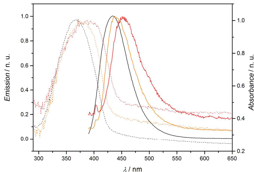
Figure 5. Absorption (dashed lines) and emission (solid line) spectra of Lu-ATA@RT (black), Lu-ATA@100 (orange), and Lu-ATA@150 (red) in acetonitrile suspension ( 5 \cdot 10^{-2} g/L). Bands are normalized for better visualization. The non-zero backgrounds results from light scattering.
