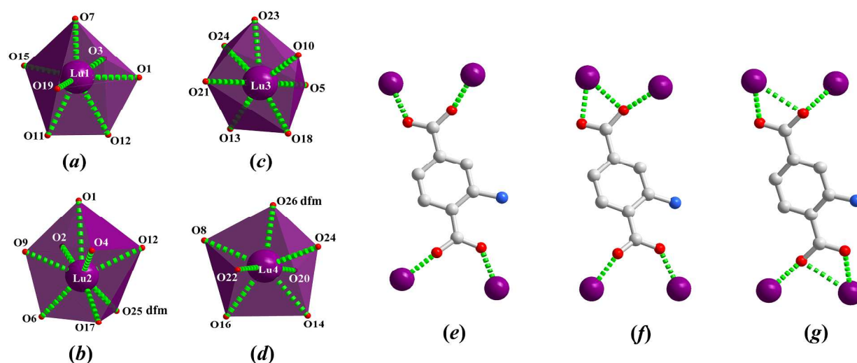
Scheme 2. Coordination environments of four Lu(III) ions in Lu-ATA@150 with corresponding atom labeling scheme: (a) and (c)–(d) monocapped and (b) bicapped trigonal truncated prisms. The coordination modes of the 2-aminoterephthalic ligands: (e) \mu_4-(\eta_1 : \eta_1 : \eta_1 : \eta_1) , (f) \mu_4-(\eta_1 : \eta_1 : \eta_1 : \eta_2) , (g) \mu_4-(\eta_1 : \eta_2 : \eta_1 : \eta_2) in Lu-ATA@150 . Hydrogens were omitted for clarity and lutetium atoms are depicted as violet spheres.
