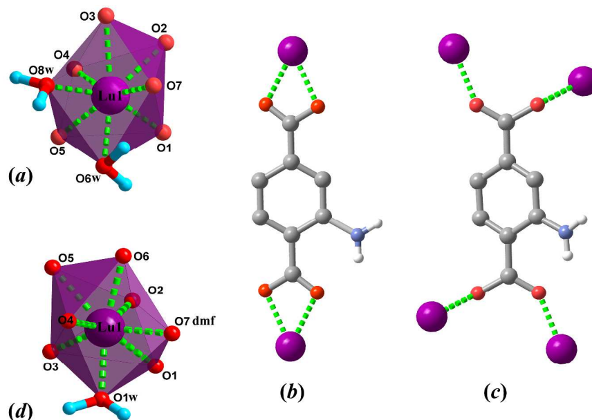
Scheme 1. Coordination environment of Lu(III) ion in (a) Lu-ATA@RT and (d) Lu-ATA@100 polymorphs, and coordination modes of the 2-aminoterephthalic ligand (b) \mu -(\eta_2 : \eta_2) and (c) \mu_4 -(\eta_1 : \eta_1 : \eta_1 : \eta_1) in both frameworks. Hydrogen atoms of benzene ring were omitted for clarity. Lutetium atoms are depicted as violet spheres.
