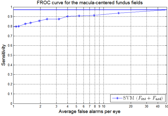
Fig. 9: FROC curve of the proposed system for the detection and classification of longitudinal retinal changes due to small red lesion applied to macula-centered fundus image pairs.
