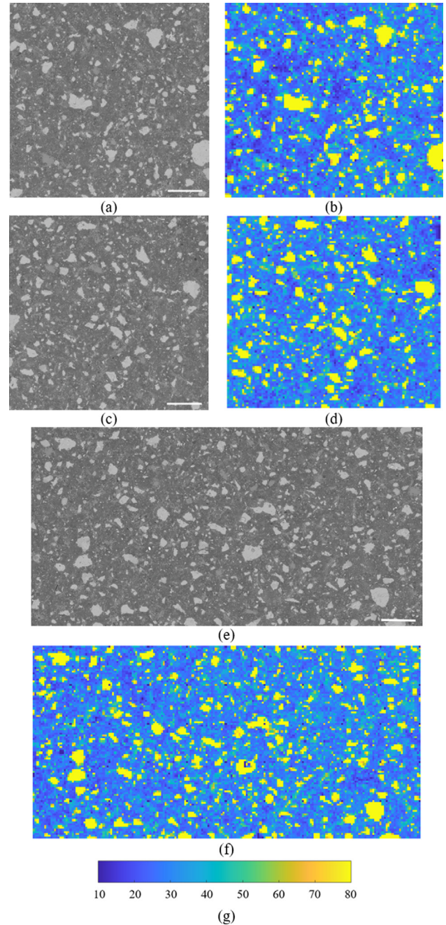
Fig. 8. Indent array and modulus map (a, c, e and b, d, f are BSE images and modulus maps of indent arrays A1, A2 and A3; g is the legend of modulus maps with the unit GPa). Scale bar = 200 \mu\text{m} .
