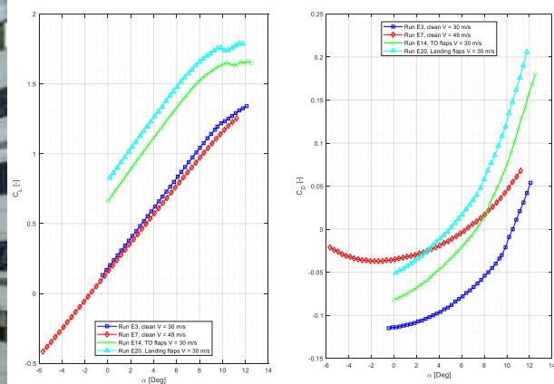
Figure 5 - Scaled aircraft with distributed electric propulsion in the wind tunnel and some results, lift and drag coefficients as a function of flap setting and air speed
