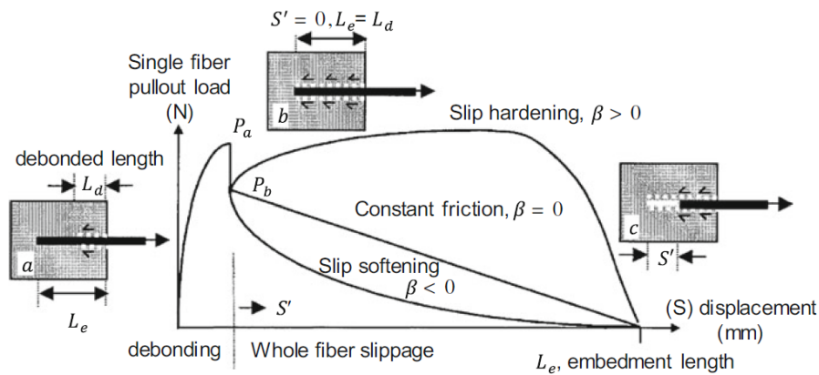
Figure 2.14 Typical pullout load P -displacement S relationship in single fiber pullout tests [137].
