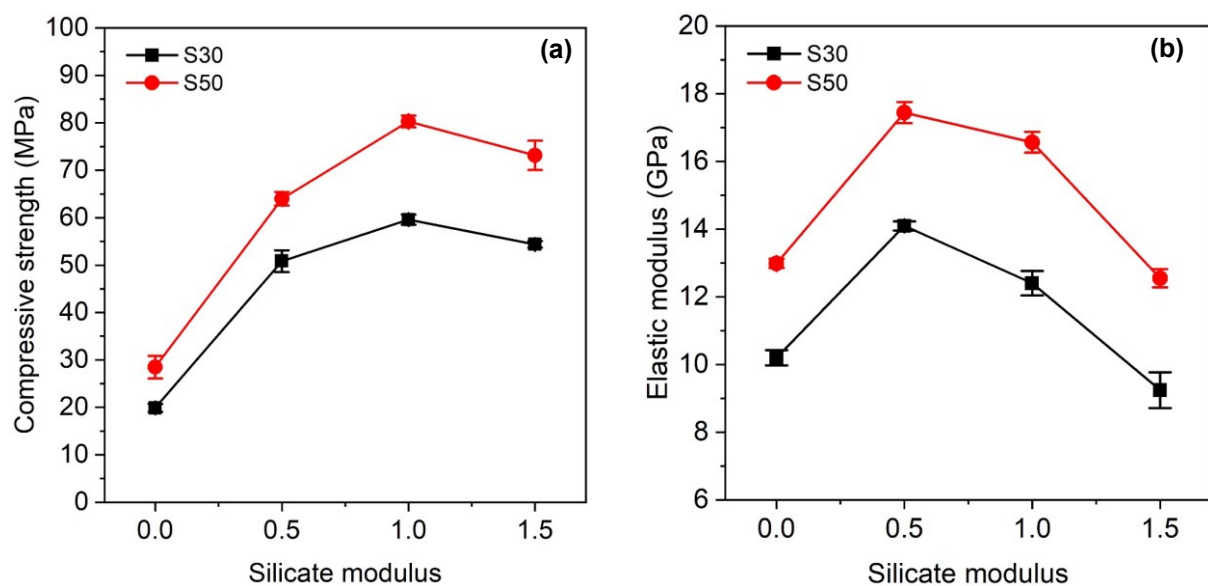
Figure 3.4 (a) Compressive strength and (b) elastic modulus of AASF pastes at 28 days as a function of activator silicate modulus 0, 0.5, 1.0, and 1.5.
