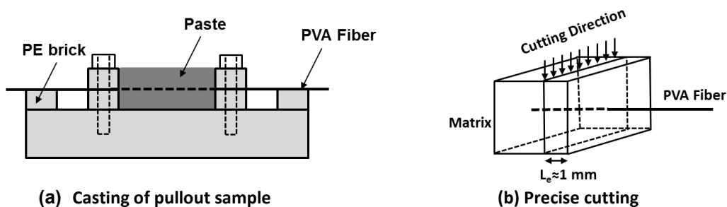
Figure 4.2 Pullout sample preparation methods: (a) casting and (b) precise cutting.
