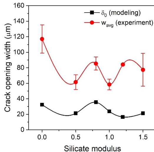
Figure 6.13 Simulated crack opening width \delta_0 by micromechanical modeling and measured loaded crack width w_{\text{avg}} as a function of activator silicate modulus
