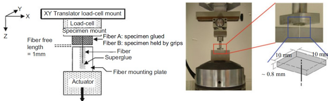
Figure 2.13 Test setup of the single fiber pullout experiment [137].
