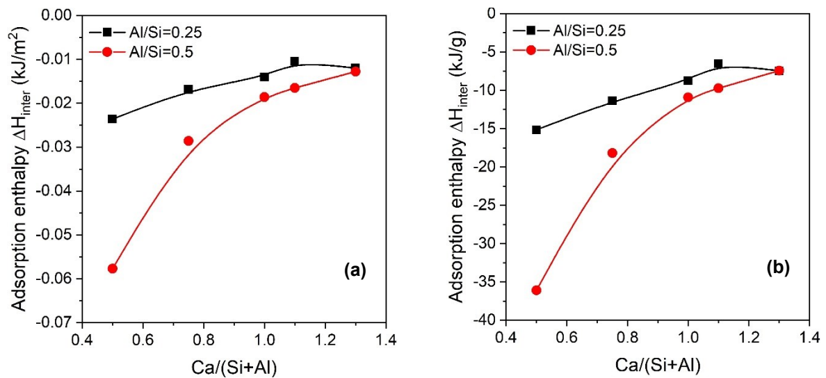
Figure 5.14 Adsorption enthalpies in (a) \text{kJ/m}^2 and (b) \text{kJ/g} attributed to the hydrogen bonds between the PVA molecule and the C-(N-)A-S-H for the composites with an Al/Si ratio of 0.25 (black squares) and 0.5 (red dots) at the considered theoretical Ca/(Si+Al) ratios.
