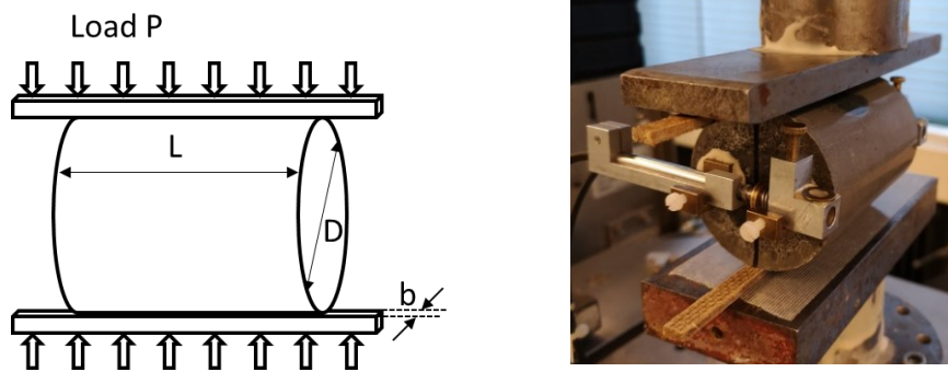
Figure 6.1 Splitting tensile test set-up.
