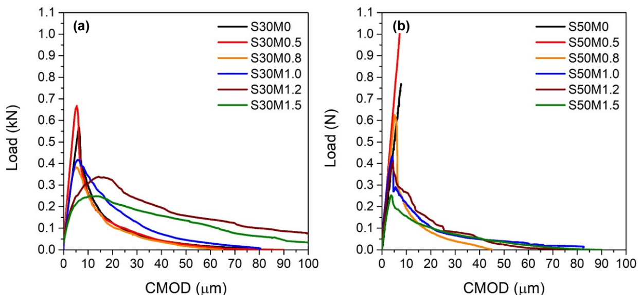
Figure 3.5 Representative Load-CMOD curves for (a) S30 pastes and (b) S50 pastes
