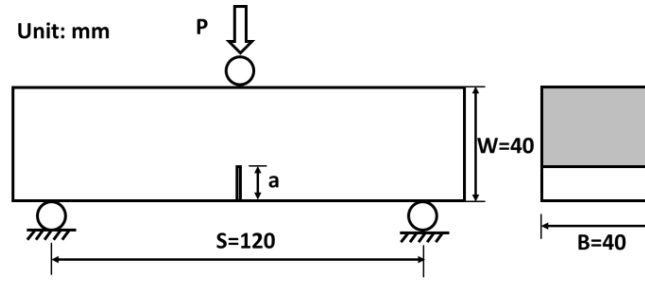
Figure 3.3 Three-point bending test configuration for single-edge notched prism specimen [129]
