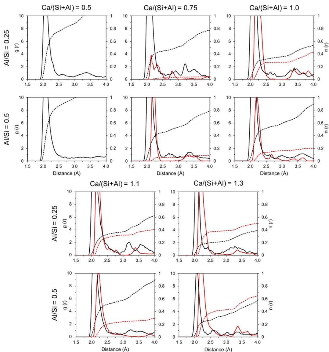
Figure 5.7 Radial distribution functions (continuous lines) and coordination numbers (dashed lines) for \text{O}_{\text{PVA-Na}} (in black) and \text{O}_{\text{PVA-Ca}} (in red) for the C-(N-)A-S-H with \text{Ca}/(\text{Si}+\text{Al}) ratios of 0.5, 0.75, 1.0, 1.1 and 1.3 at \text{Al}/\text{Si} ratios of 0.25 and 0.5.
