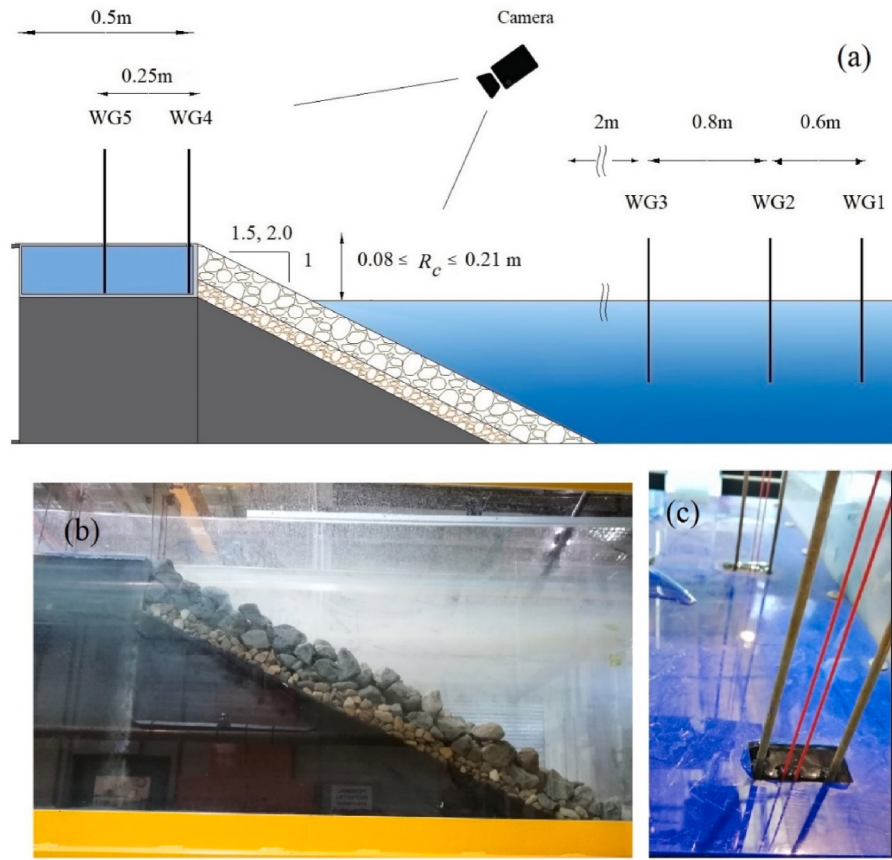
Fig. 2. (a) and (b): Cross section of the model; (c): Wave gauges on the crest of the structure.
