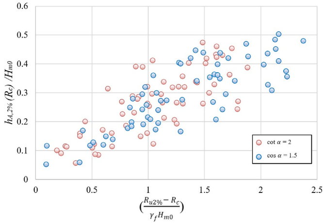
Fig. 4. Dimensionless difference between R_{u2\%} and the crest free board against measured h_{A,2\%}(R_c)/H_{m0} for different slopes of the structure.
