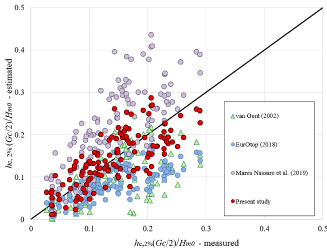
Fig. 7. Measured vs estimated h_{c,2\%}(x_c = G_c/2)/H_{m0} using existing formulas for dikes and rubble mound breakwaters, and newly proposed one (present study) for rock-armoured seawall.
