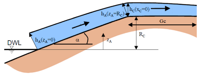
Fig. 1. Definition of overtopping flow layer profile by Schüttrumpf and van Gent (2003).
