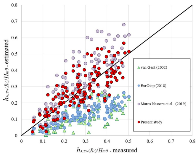
Fig. 5. Estimated vs measured h_{A,2\%}(R_c)/H_{m0} ( \gamma_f = 0.55 ), using existing formulas for dikes and rubble mound breakwaters, and newly proposed one for rock-armoured seawall.
