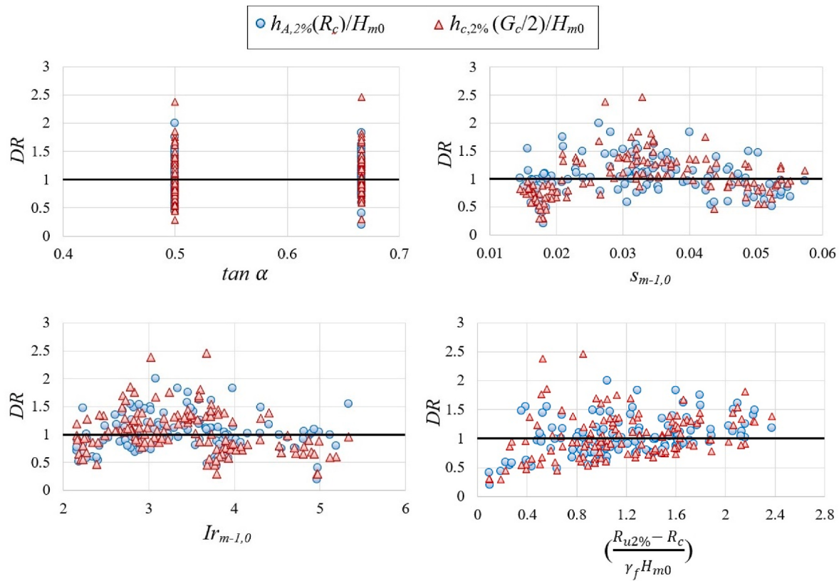
Fig. 8. Discrepancy ratios of estimated h_{A,2\%}(R_c)/H_{m0} and h_{c,2\%}(x_c = G_c/2)/H_{m0} of the proposed formulas against seaward slope of structure (top-left); wave steepness (top-right), Iribarren number (bottom-left) and dimensionless difference of wave run-up and the crest freeboard.
