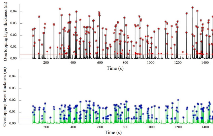
Fig. 3. Recorded wave overtopping layer thickness at the seaward edge (top) and the middle (bottom) of the crest (Each circle corresponds to the detection of an individual overtopping event and horizontal lines show down-crossing threshold). H_{m0} = 0.1 m, T_p = 1 s.
