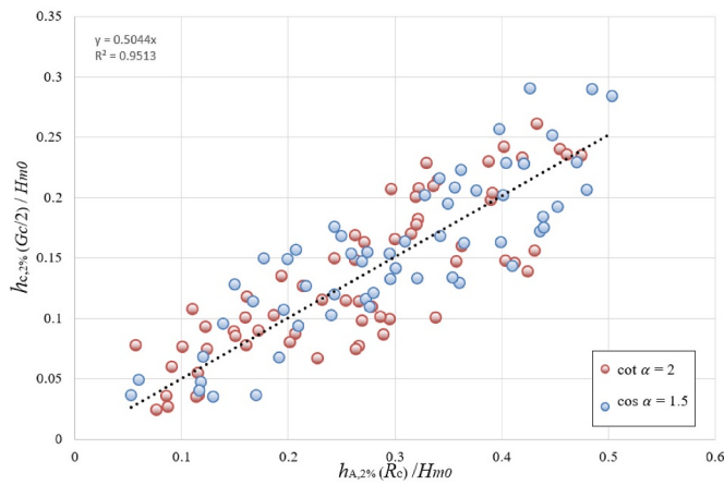
Fig. 6. Measured h_{A,2\%}(R_c)/H_{m0} against h_{c,2\%}(x_c = G_c/2)/H_{m0} .
