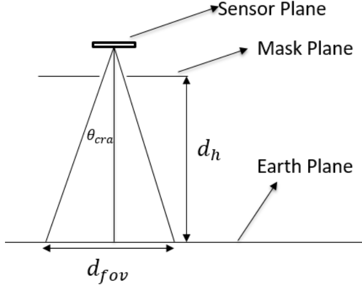
Figure 2.6: Field of View Calculation
