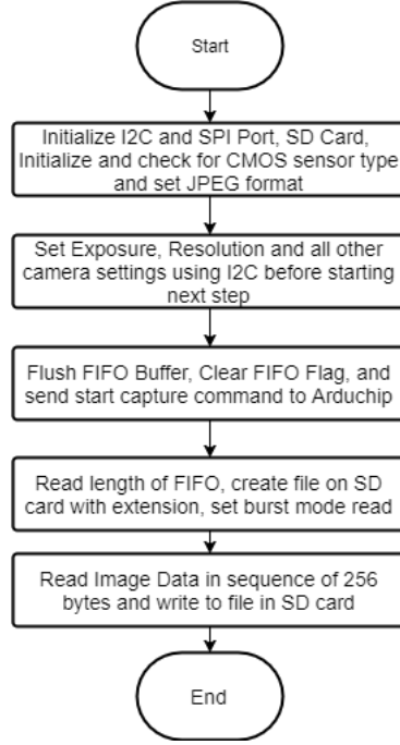
Figure 4.3: Software Flow used for image acquisition from CMOS sensors
