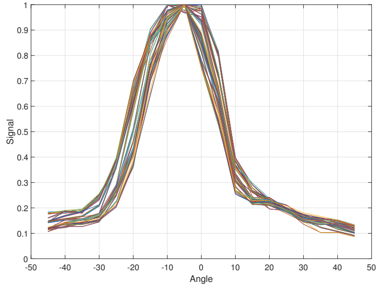
Figure 5.8: Response for 100 different offset pixel positions from central diffraction pattern in X-direction
