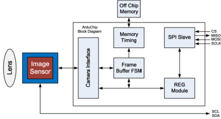
Figure 4.1: Camera Architecture of Arducam Mini OV2640 Camera Module[17]
