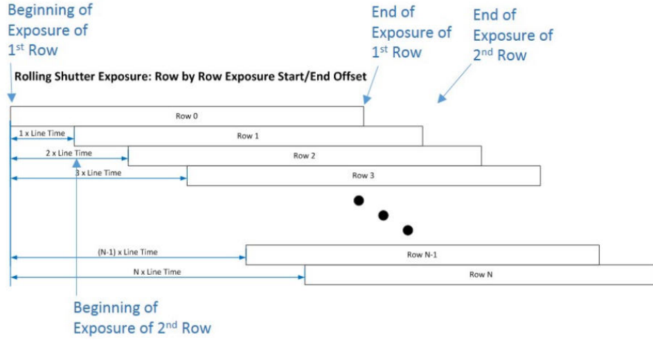
Figure 4.4: Rolling Shutter Operation on OV2640[8]
