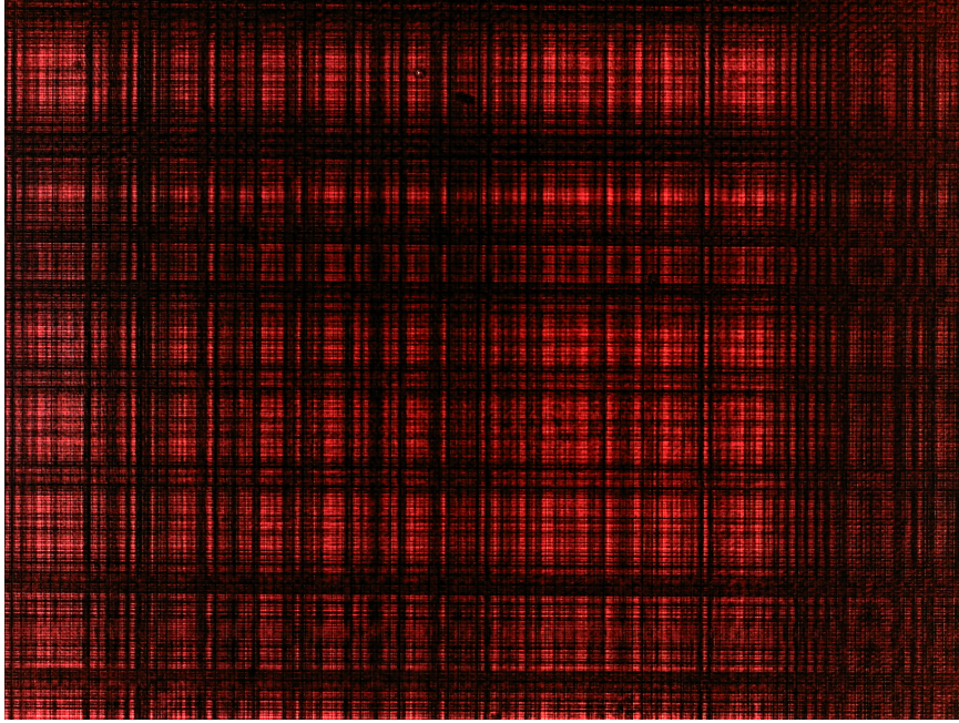
Figure 6.8: Doubly Toeplitz mask imaged by OV5642
