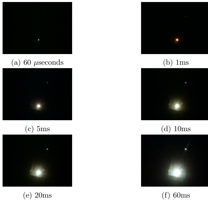
Figure 4.7: Images of a laser beam caught in different exposure times(with lens)
