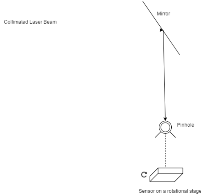
Figure 5.1: Experimental Setup for detection of acceptance cone
