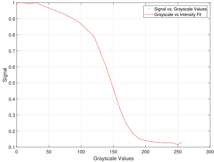
Figure 6.5: Grayscale vs intensity of light received by the CMOS sensor.
