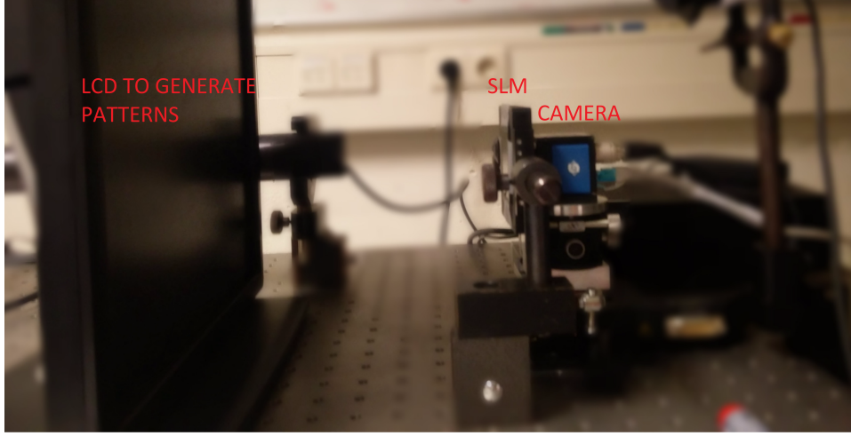
Figure 7.1: Setup for Intial Experiments
