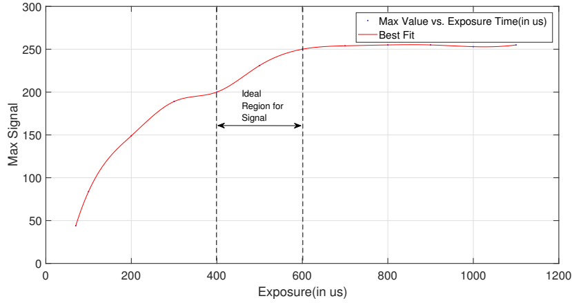
Figure 5.3: Response for different Exposure values in microseconds
