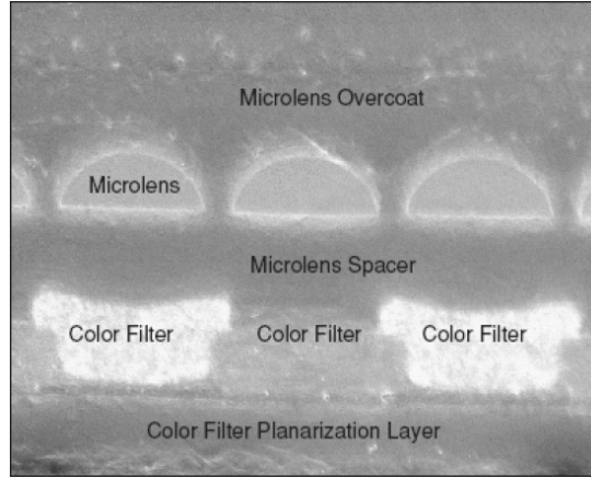
(b) Micro lens array and other components in a image sensor
