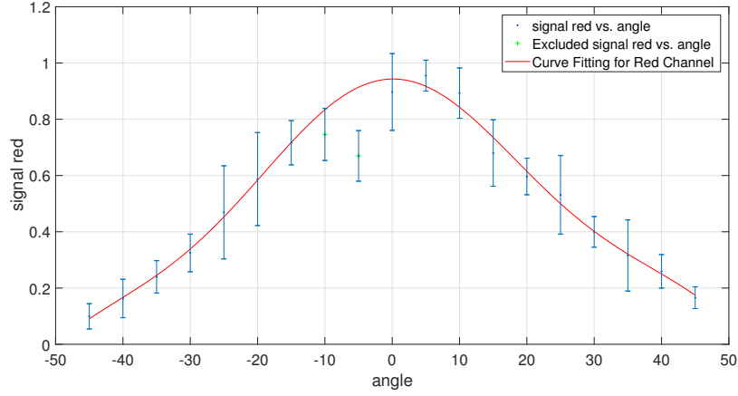
Figure 5.4: Response for Red Channel in Initial Experiment
