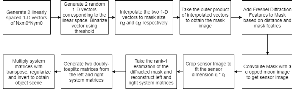
Figure 3.2: Simulation-Flow separable mask
