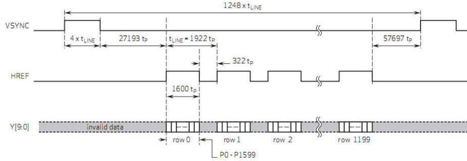
Figure 4.5: Shutter Timing Diagram of OV2640[8]
