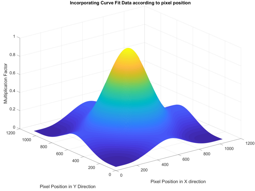
Figure 5.12: Fitted Curve Data into simulation
