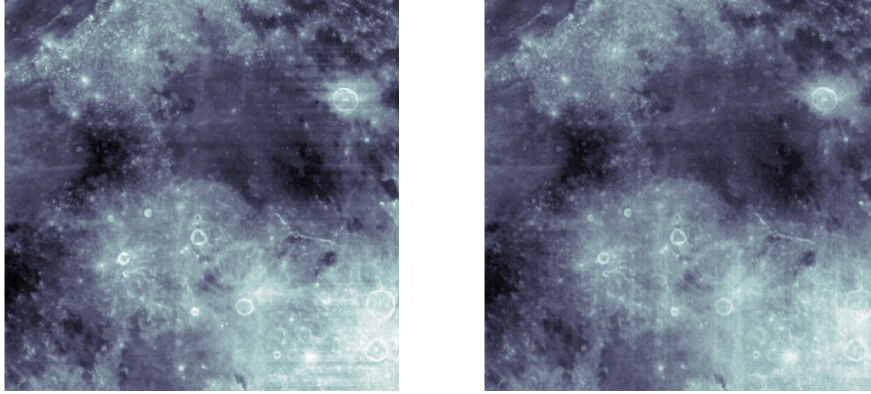
Figure 3.6: The figure shows the reconstruction with and without fresnel diffraction effects for a separable mask using equation 3.15. We are able to obtain \text{PSNR} = 57.85 without diffraction effects. It can be seen that we can obtain reconstructions even in the presence of diffraction effects with \text{PSNR} = 57.93
