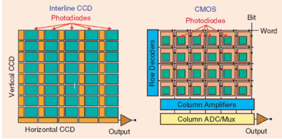
(a) Readout architectures of CMOS and CCD
