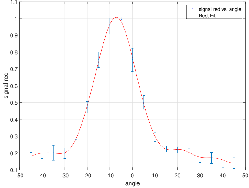
Figure 5.11: Finalized Red Channel Response for Different Data Sets
