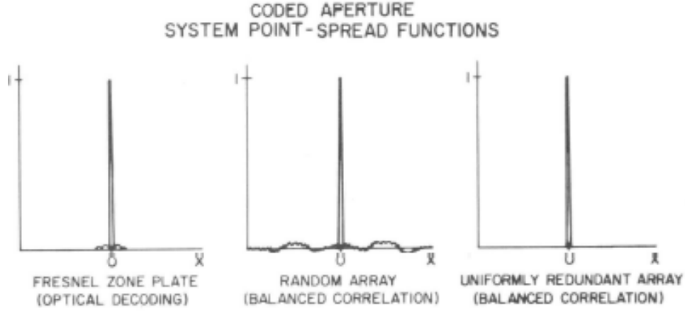
Figure 2.14: Point Spread function of different masks[27]
