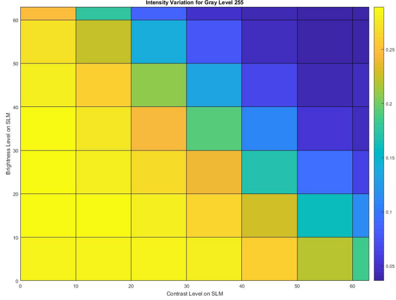
Figure 6.4: Effect of brightness and contrast on intensity for grayscale 255
