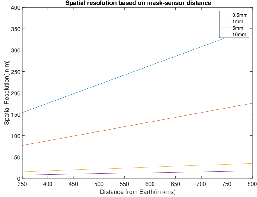
Figure 5.14: Relation between Spatial resolution and mask-sensor distance for sensor OV2640
