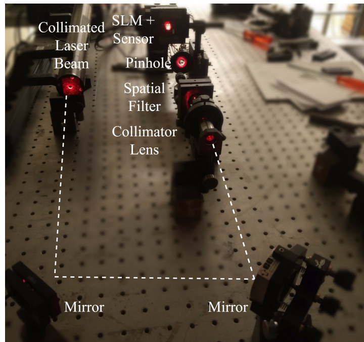
Figure 6.1: Experimental Setup to image mask
