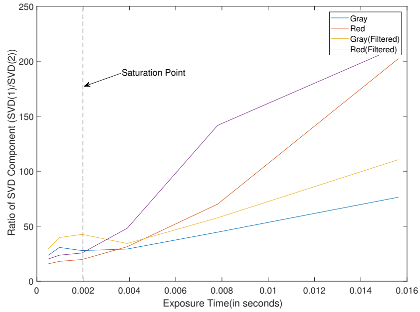
Figure 6.10: Impact of Exposure Time on Singular Values
