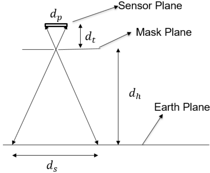
Figure 2.5: Spatial Resolution Calculation
