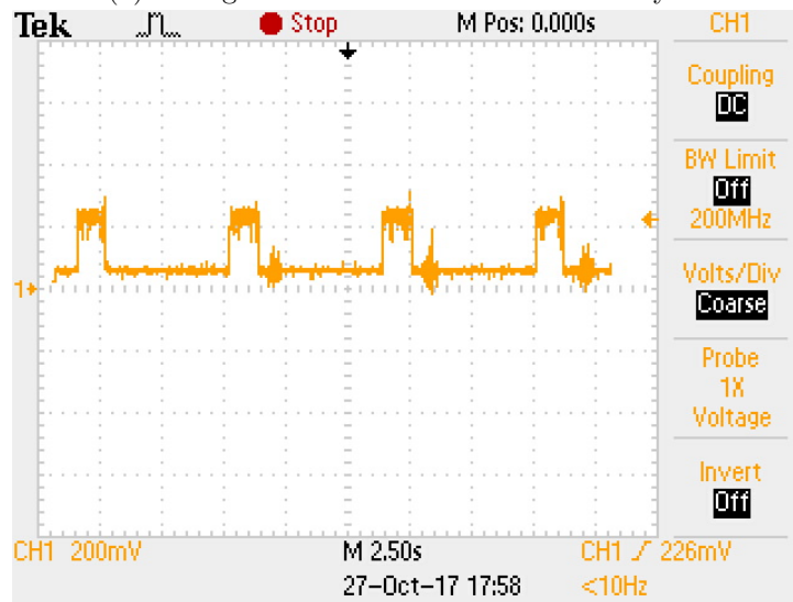
(b) Voltage across resistor when using GPIO_PWDN_MASK
