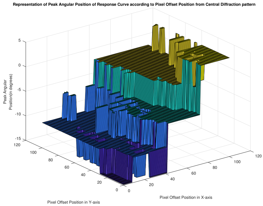
Figure 5.10: Peak Angular Positions for different Pixels
