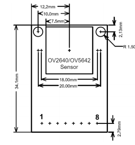
Figure 8.2: Dimensions of both OV5642 and OV2640 camera modules
