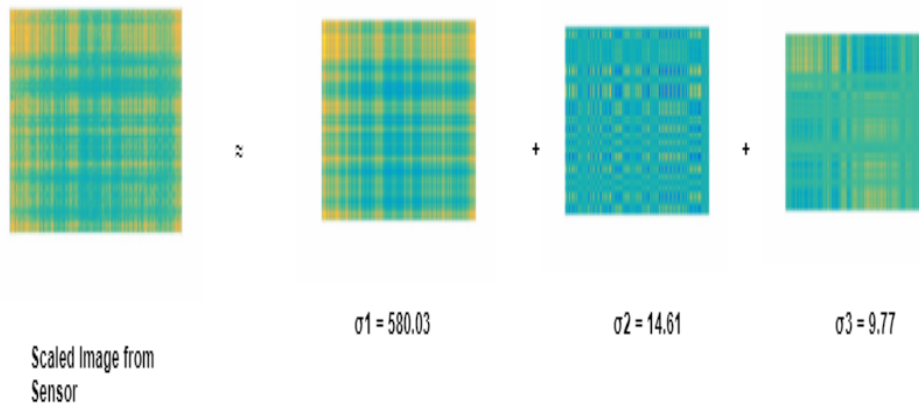
Figure 6.11: Decomposition of best data set(Ratio of first to second component = 39.70 )
