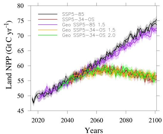
Figure 7. Annual land-accumulated NPP ( \text{GtC yr}^{-1} ) in baseline and SAG scenarios and ensemble members (different colors are indicated in legend). The shaded areas are significant with 95 % confidence, assuming normally distributed data.
