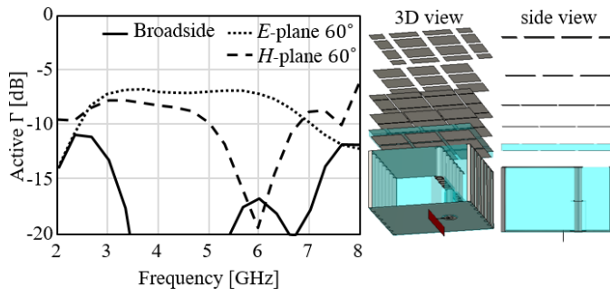
Fig. 7. Active reflection coefficient for broadside and scanning to 60° in the E-plane for the single-polarized unit cell in the inset.
