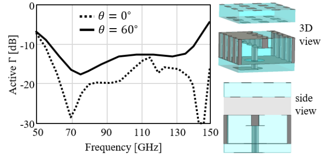
Fig. 6. Active reflection coefficient for broadside and scanning to 60° in the E-plane for the unit cell in the inset.
