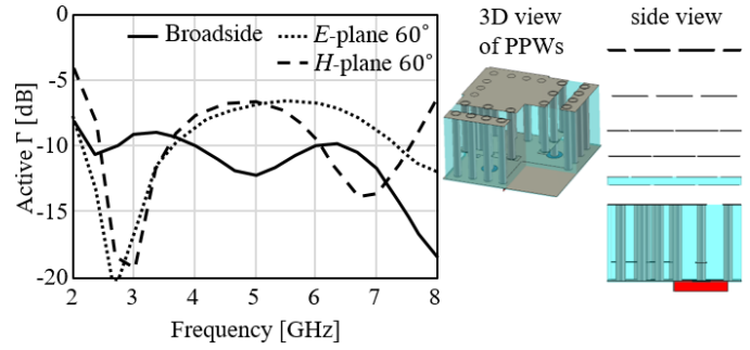
Fig. 9. Active reflection coefficient for broadside and scanning to 60° in the E-plane for the dual-polarized unit cell in the inset.
