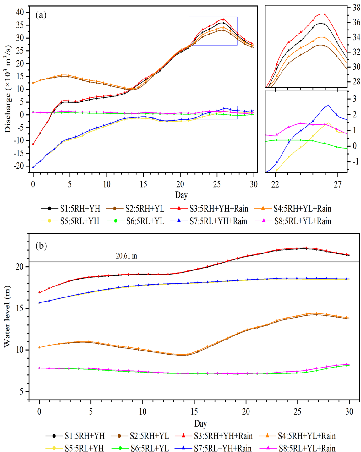
FIGURE 11 Outflow conditions of the Lake under different scenarios during wet season: (a) flow discharge ( 10^3 \text{ m}^3/\text{s} ), (b) water level. 5RH and 5RL are for the maximum and minimum discharge conditions of the five major inflowing rivers, respectively; YH and YL represent the maximum and minimum discharge conditions of the Yangtze River, respectively; precipitation represents the maximum areal rainfall for the Lake catchment
