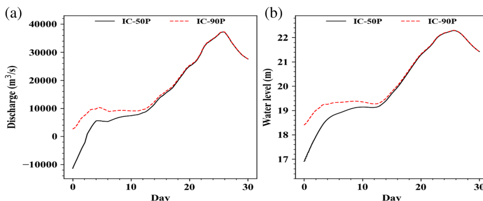
FIGURE 13 Impact of the initial conditions on the Lake outflow discharge: (a) flow discharge ( \text{m}^3/\text{s} ), (b) water level (m). IC-50P, IC-90P are for the 50, 90 percentile of the water level at Hukou, respectively
