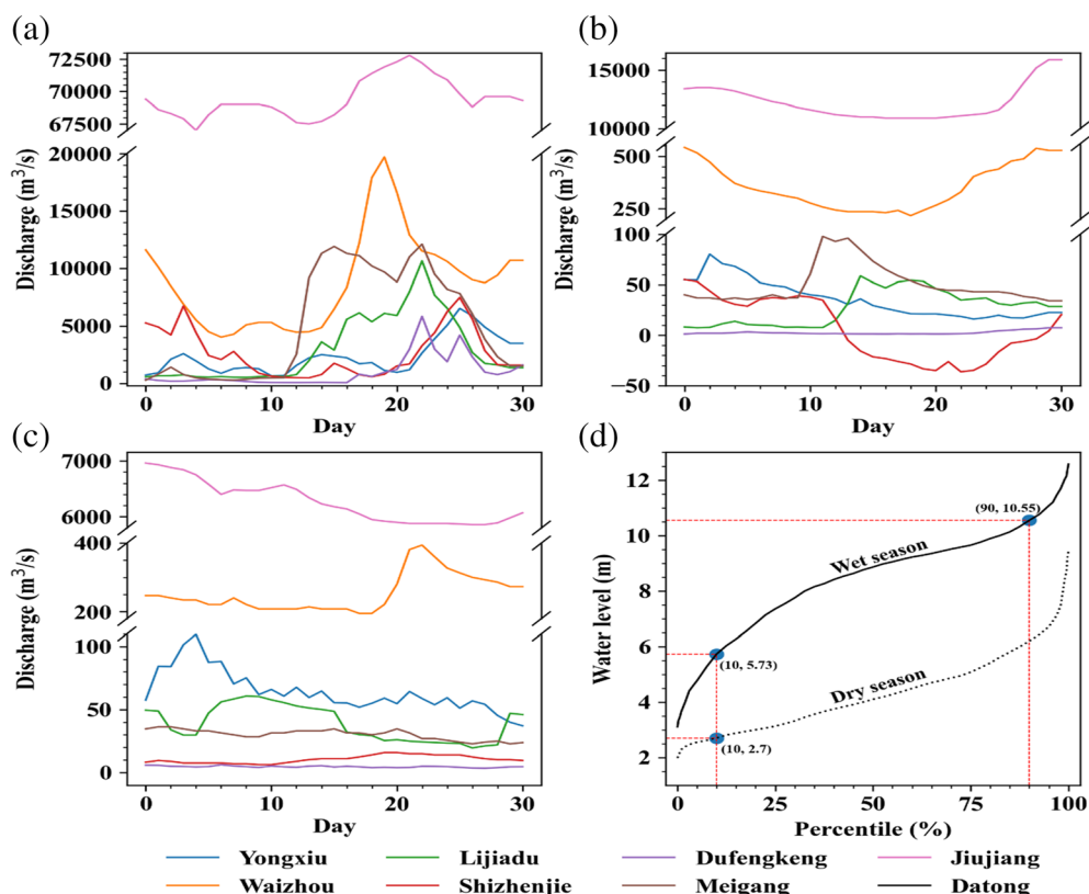
FIGURE 10 Boundary conditions of the 1D- and 2D-coupled hydrodynamic model: (a) maximum flow process in wet season ( \text{m}^3/\text{s} ), (b) minimum flow process in wet season ( \text{m}^3/\text{s} ), (c) minimum flow process in dry season ( \text{m}^3/\text{s} ), and (d) lower boundary condition at Datong (m)
