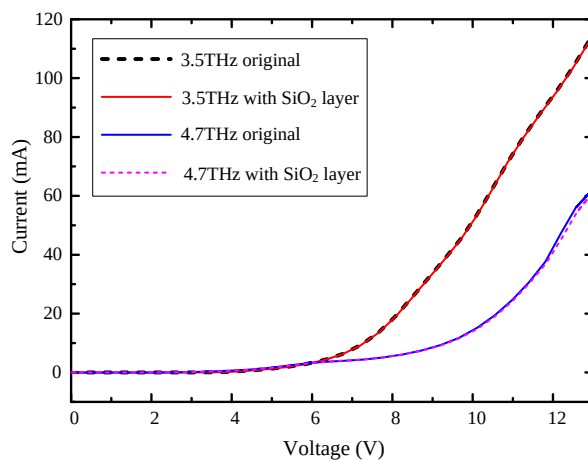
Figure 4.4. Measured I-V curves of both lasers before and after \text{SiO}_2 deposition.
