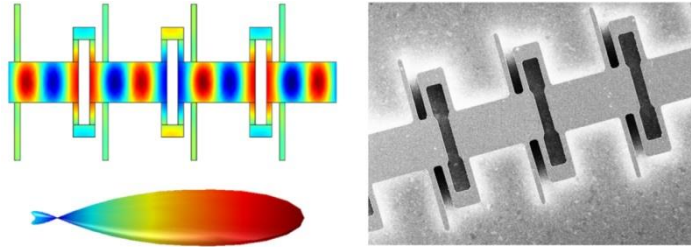
Figure 2.10. Electric field distribution and far-field radiation pattern (a) together with an SEM photo of a unidirectional third-order DFB THz QCL [32]
