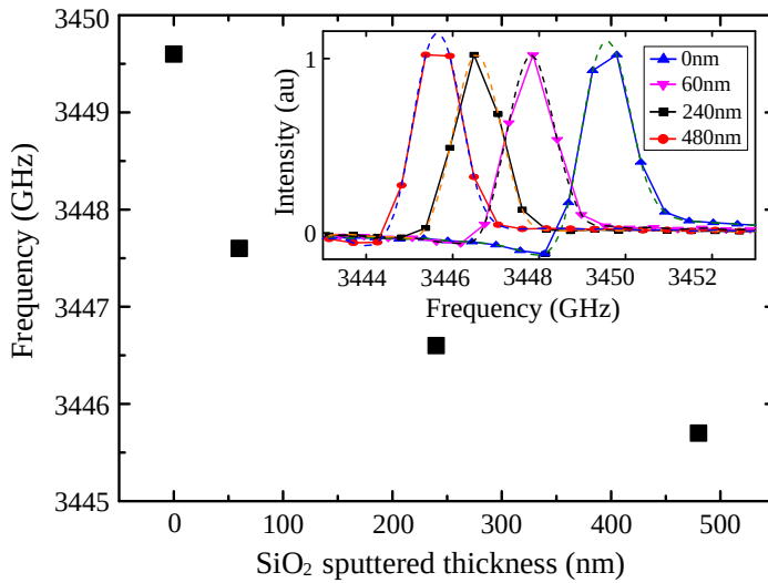
Figure 4.3. Measured frequency as a function of the thickness of the sputtered \text{SiO}_2 on the 3.5 THz QCL. The thickness is zero when there is no \text{SiO}_2 . Inset: Normalized measured FTS spectra without and with three different thicknesses of the sputtered \text{SiO}_2 . Dashed are fitted curves to find the central frequencies.
