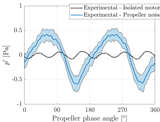
Fig. 3 Experimental average time history of the acoustic pressure fluctuations of the propeller at \phi = 0^\circ compared to the one of the isolated motor. Blue shades show maximum and minimum level deviation with respect to the pressure time-history acquired.
