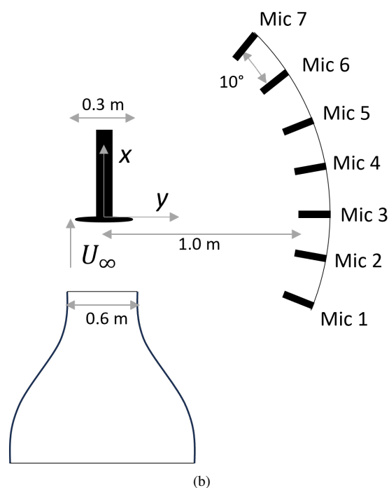
Fig. 1 Experimental setup and geometry.
