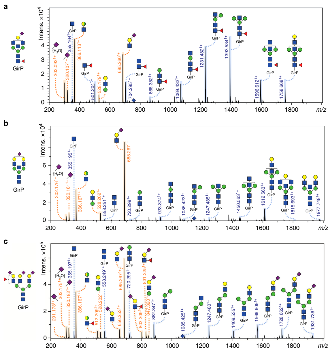
Fig. 3 CE-ESI-MS/MS fragmentation spectra of derivatized and labelled N-glycans from TPNG. The following precursor ions were fragmented: a 760.9603 + (H4N5F1S 2.6 1), b 1148.9392 + (H5N5S 2.6 1) and c 1072.0763 + (H6N5F1S 2.3 1S 2.6 2). The Y-ion fragmentation pattern is annotated in blue and the B-ion fragmentation pattern is annotated in orange. Blue diamond: precursor ion, blue square: N-acetylglucosamine, green circle: mannose, yellow circle: galactose, red triangle: fucose, right pointing pink diamond: α2,6-linked N-acetylneuraminic acid, left pointing pink diamond: α2,3-linked N-acetylneuraminic acid, GirP: Girard's reagent P label. *The presence of an antennary fucose in combination with an α2,6-linked sialic acid is likely, for a large part, due to fucose migration during MS analysis 36
