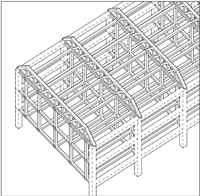
STRUCTURAL DIAGRAM
