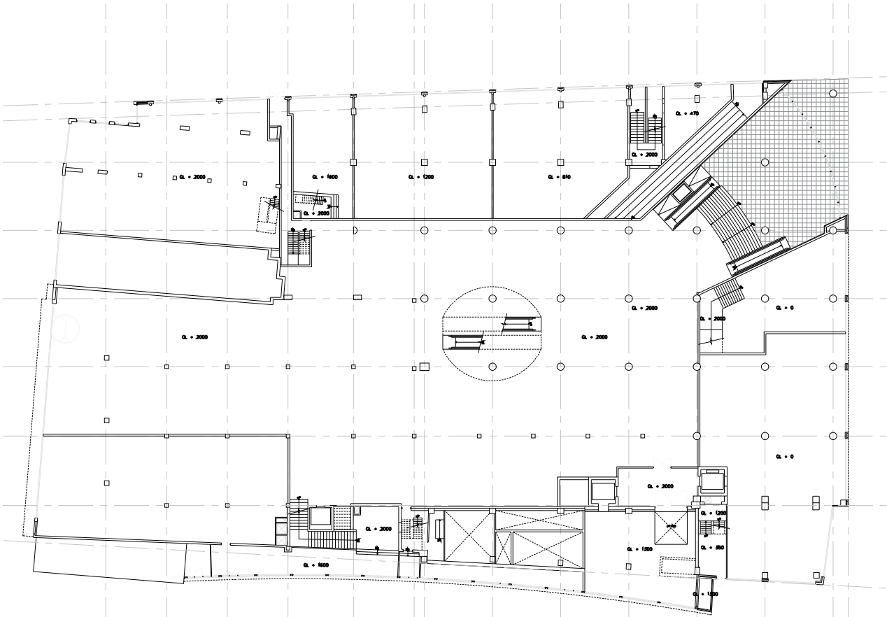
Illustration: Axon view of former V&D building in Dordrecht, section, plan, based on SBT research(2020)
