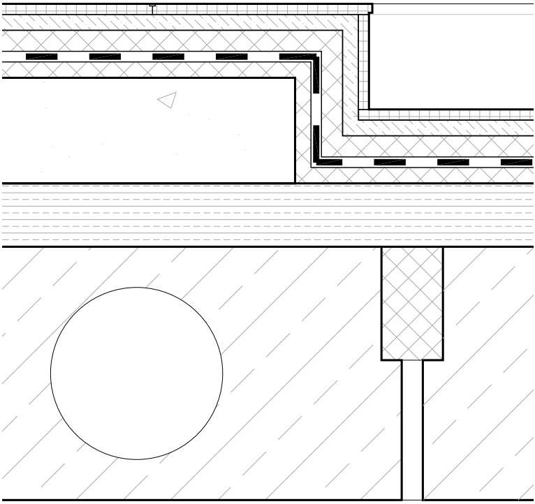
SLAB DETAIL
