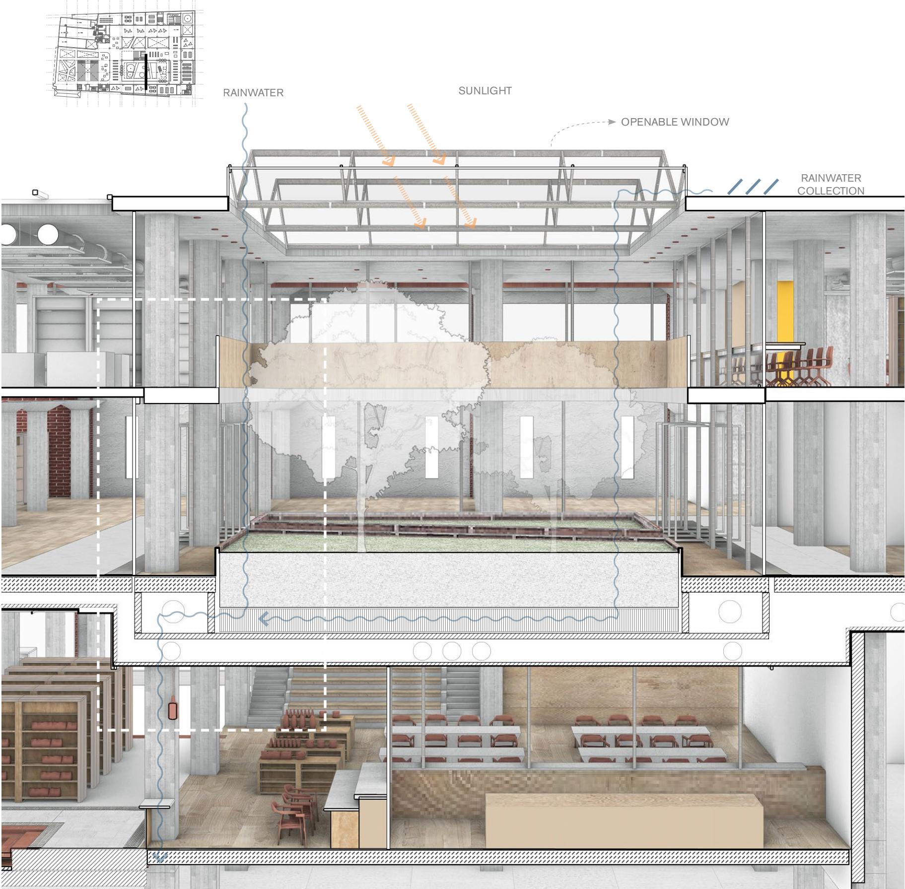
SECTION OF FLOATING GARDEN
