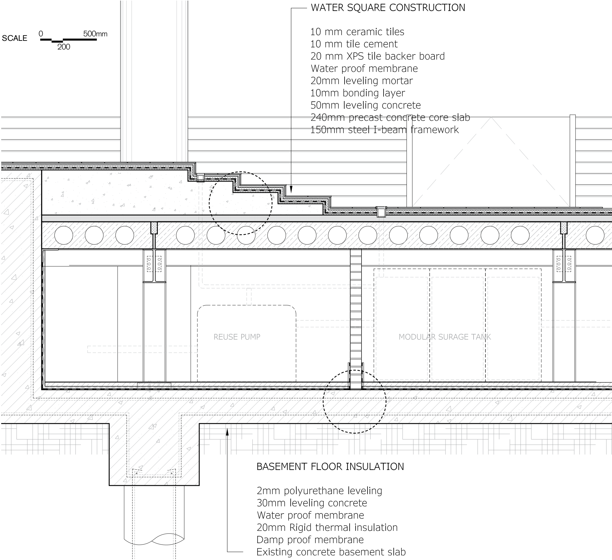
DETAIL OF WATER SQUARE
