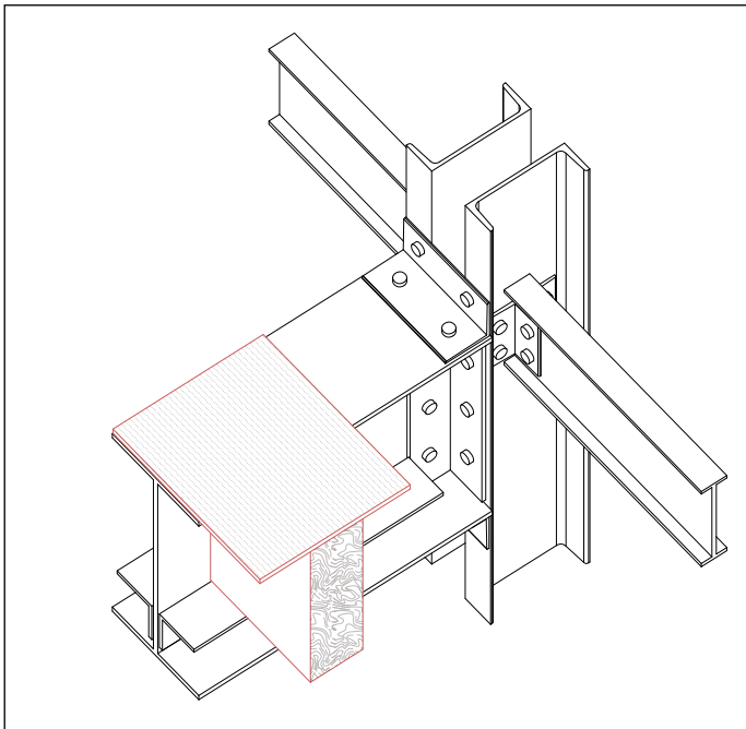
STRUCTURAL DIAGRAM
