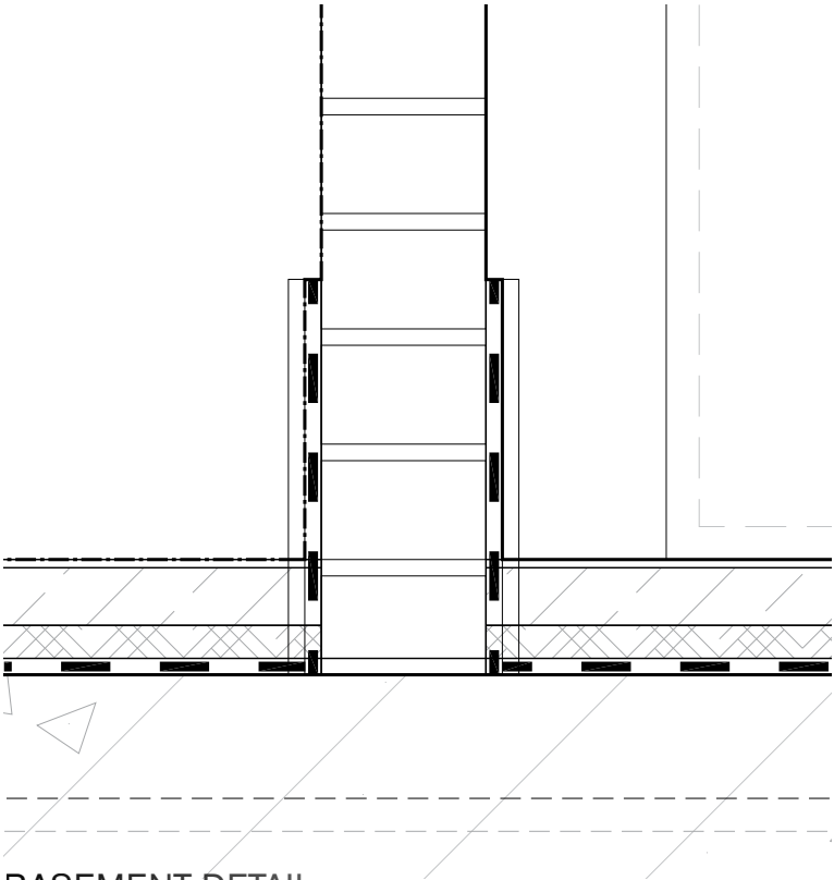
BASEMENT DETAIL
