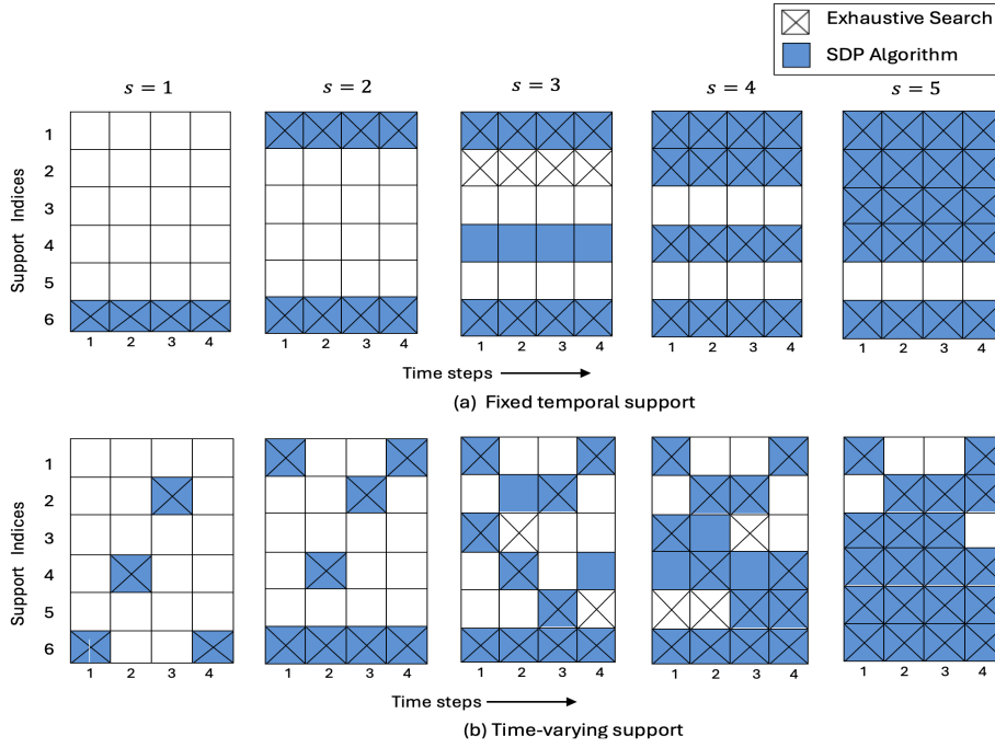
Fig. 2. Sparse supports obtained from our SDP-based algorithm and the exhaustive search. Horizontal axis represents time steps from k = 0, \dots, N - 1 . k^{\text{th}} column of each table represents support vector of the input u_k .
