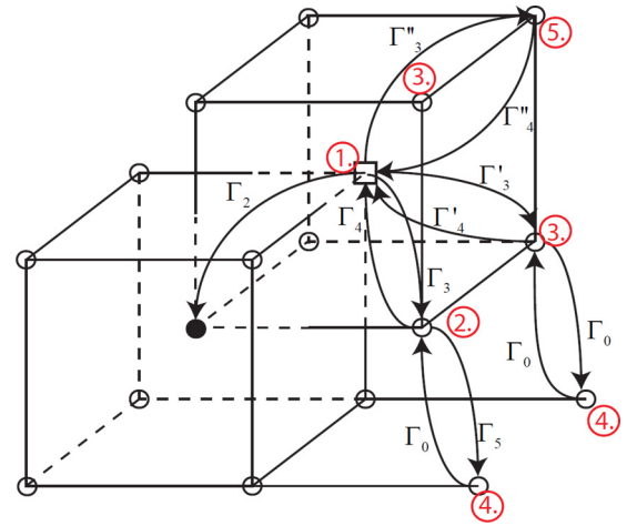
FIG. 1. The nine-frequency model by Le Claire [70,71]. Each distinct jump frequency is indicated, with the red numbers indicating the nearest neighbor with respect to the impurity atom. \Gamma_2 concerns the impurity trading places with the vacancy, \Gamma_3 concerns an iron atom that is a second neighbor of the impurity exchanging with a vacancy and thereby becoming a nearest neighbor to the impurity, \Gamma_4 is the reverse of \Gamma_3 , \Gamma_{3'} is a jump whereby an iron atom changes from a first to a third neighbor of the impurity, \Gamma_{4'} is the reverse of \Gamma_{3'} , an iron atom jumping from first to fifth impurity neighbor is \Gamma_{3''} , and \Gamma_{4''} is the reverse of \Gamma_{3''} . All other jump frequencies are assumed to be unaffected by the presence of a substitutional solute and are assumed to take the same value as the one in pure iron bulk \Gamma_0 .
