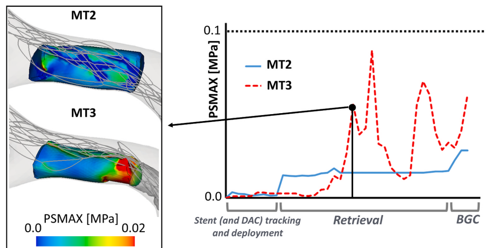
Fig. 7. PSMAX over time during the MT2 and MT3 simulations. A comparison of the PSMAX fields on the thrombus is shown in an instant during the retrieval phase. Discontinuous black line: PSMAX threshold for fibrin-rich thrombi. Fragmentation does not occur during the simulation for both models.
