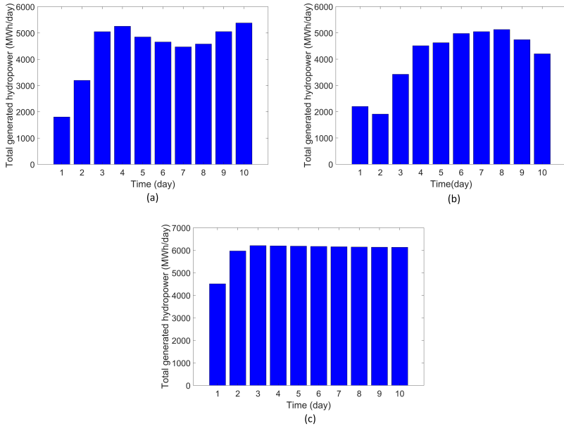
Figure 5.7: (a-c) Total generated hydropower under DR 1 (a), 2 (b) and 3 (c).
