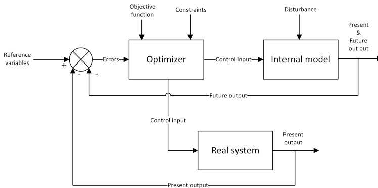
Figure 1.4: Structure diagram of Model Predictive Control
