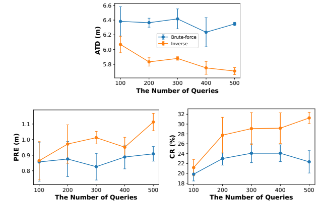
Figure 17: ATD, PRE, and CR under brute-force sampling attack and our inverse attack in the black-box scenario. The attack is planned using Trajectron++ predictor and evaluated on the AgentFormer model.
