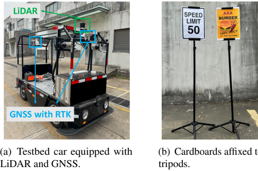
Figure 18: Physical-world experiment setup.
