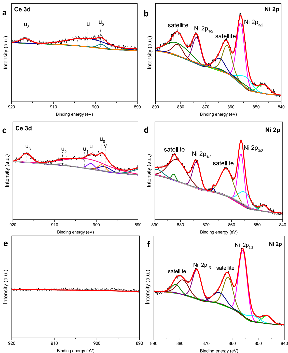
Fig. 9. (a) Ce 3d XPS spectra in 5%Ni2.5%Ce13X; (b) Ni 2p XPS spectra in 5%Ni2.5%Ce13X; (c) Ce 3d XPS spectra in 5%Ni5%Ce13X; (d) Ni 2p XPS spectra in 5%Ni5%Ce13X; (e) Ce 3d spectra in 5%Ni13X, (f) Ni 2p XPS spectra in 5%Ni13X.
