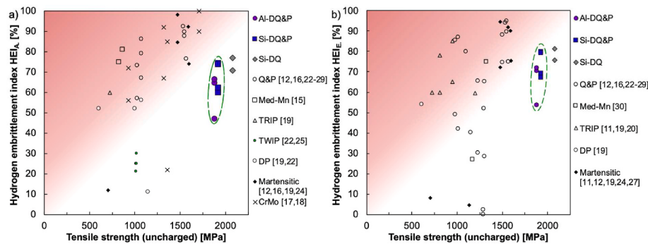
Fig. 8. Comparison of HE susceptibility of high-strength steels with nominal uncharged tensile strength and a) hydrogen embrittlement index from area reduction HEI_A , and b) hydrogen embrittlement index from loss of elongation HEI_E . Green dashed circles highlight the results with DQ&P steels. External data: Q&P [12,16,22–29], Med-Mn: [15,30], other TRIP steels [11,19,20], TWIP [22,25], DP [19,22], Martensitic: [11,12,19,24,27], and CrMo [17,18] steels. (For interpretation of the references to colour in this figure legend, the reader is referred to the Web version of this article.)
