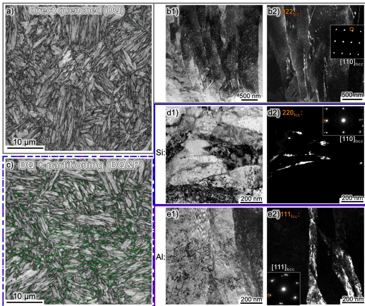
Fig. 3. Microstructure of a) essentially lath-martensitic Si-DQ in EBSD image quality map, b1) bright field TEM image of the lath structure, b2) dark field image of inter-lath residual austenite exited with a 022 fcc spot. Martensitic-austenitic microstructures in c) in image quality map of Al-DQ&P with retained austenite locations shown in green, Si-DQ&P laths and RA films in d1)-d2), and Al-DQ&P with thicker RA films in e1)-e2). (For interpretation of the references to colour in this figure legend, the reader is referred to the Web version of this article.)
