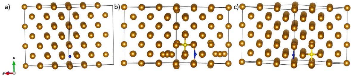
Fig. 2. 3 \times 3 \times 3 supercells for fcc-Fe (golden) with a) H_{int} (blue) at the octahedral position, b) H_{int} as the first nearest neighbour of a C_{int} (yellow), and c) H_{int} and C_{int} as second nearest neighbours. (For interpretation of the references to colour in this figure legend, the reader is referred to the Web version of this article.)
