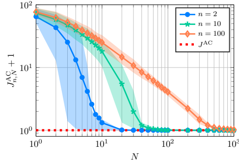
FIG. 4. The quantity J_{n,N}^{AC} is computed using (4.5). The optimal value J^{AC} is approximated by n = 10^3 and N = 10^6 , which amounts to 0 as also reported in [43].
