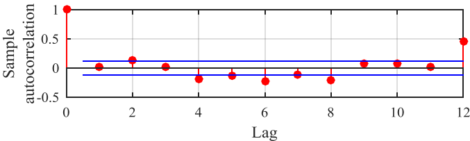
Fig. 1. ACF and PACF of residuals without seasonality
