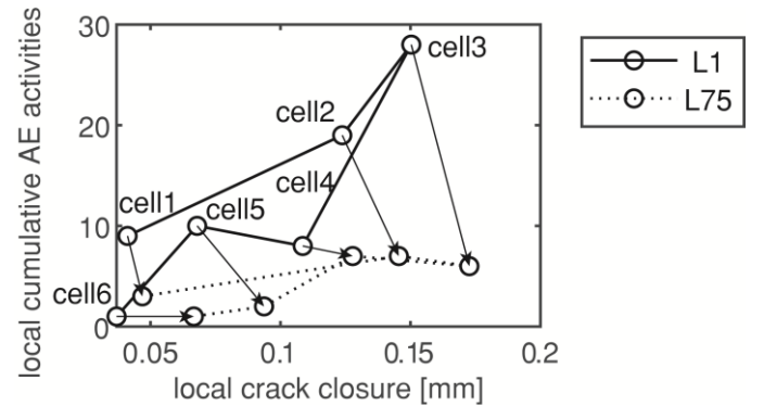
Figure 10. Local cumulative AE activities vs local crack closure in L1 and L75.
