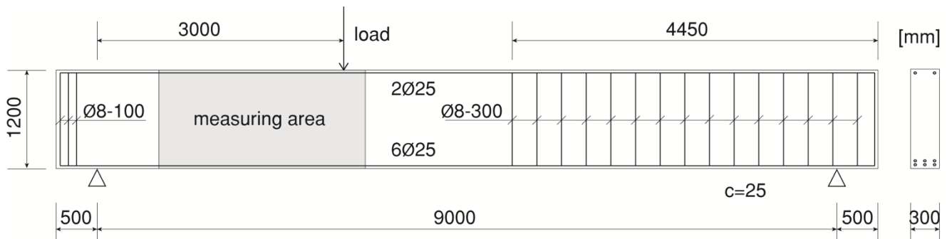
Figure 1. Beam configurations.
