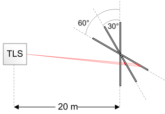
Figure 3: Top view of the measurement setup 1, with schematic depiction of horizontal rotations of the plate using the goniometer. A representative laser beam is depicted in red.
