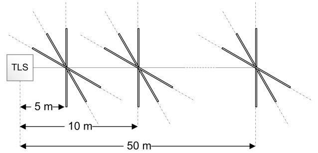
Figure 5: Top view of the measurement setup 2, with schematic depiction of distance placement of the plate with respect to the TLS.
