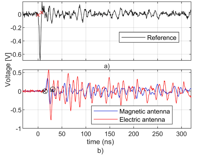
Fig. 13. a) HFCT measured reference pulse and b) Magnetic and Electric antennas measurements with their integration time limits (black crosses and circles) [16].
