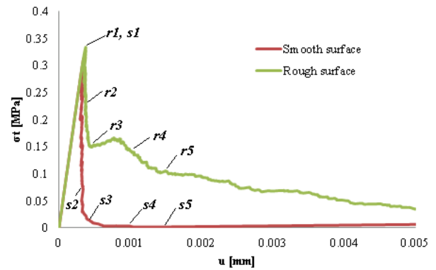
Figure 5: Tensile stress vs. vertical (opening) displacement for rough and smooth surface
