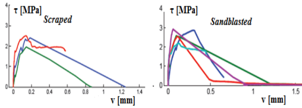
Figure 12: Experimental results for shear bond test [18]
