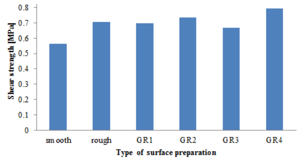
Figure 14: Shear strength for different surface preparation
