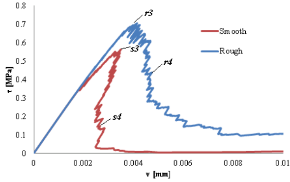
Figure 11: Shear stresses plotted against horizontal (sliding) displacement.
