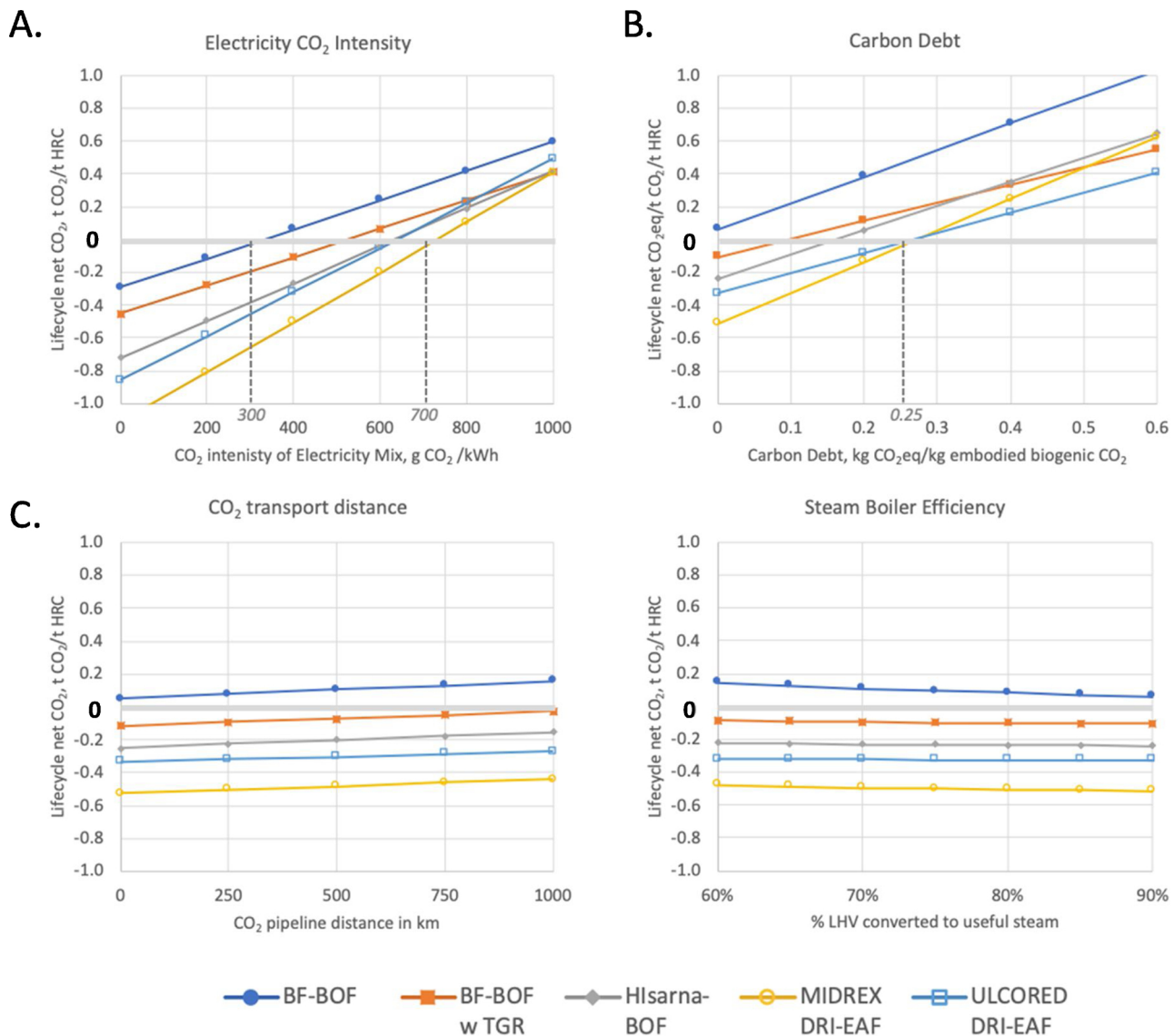
Fig. 5. Sensitivity analysis of electricity carbon intensity (A), biomass carbon debt (B), CO 2 transport distance (C), and steam boiler efficiency (D) in the cases of high bioenergy and high CCS use for all technologies.
