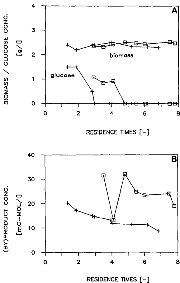
Figure 4.4A,B. Growth by a C. roseus suspension culture in a glucose-limited chemostat stirred with a 4.5 cm turbine impeller at agitation speeds of 2.1 and 16.7 \text{s}^{-1} , dilution rate= 0.006 \text{ h}^{-1} . A. biomass dry-weight; residual glucose [ \text{g}\cdot\text{l}^{-1} ]. B. (by)product [ \text{mC}\cdot\text{mol}\cdot\text{l}^{-1} ]. ( \square ) 2.1 \text{s}^{-1} , D=0.0060 \text{ h}^{-1} ; (+) 16.7 \text{s}^{-1} , D=0.0056 \text{ h}^{-1}
