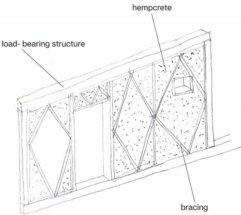
stability prefabricated elements
