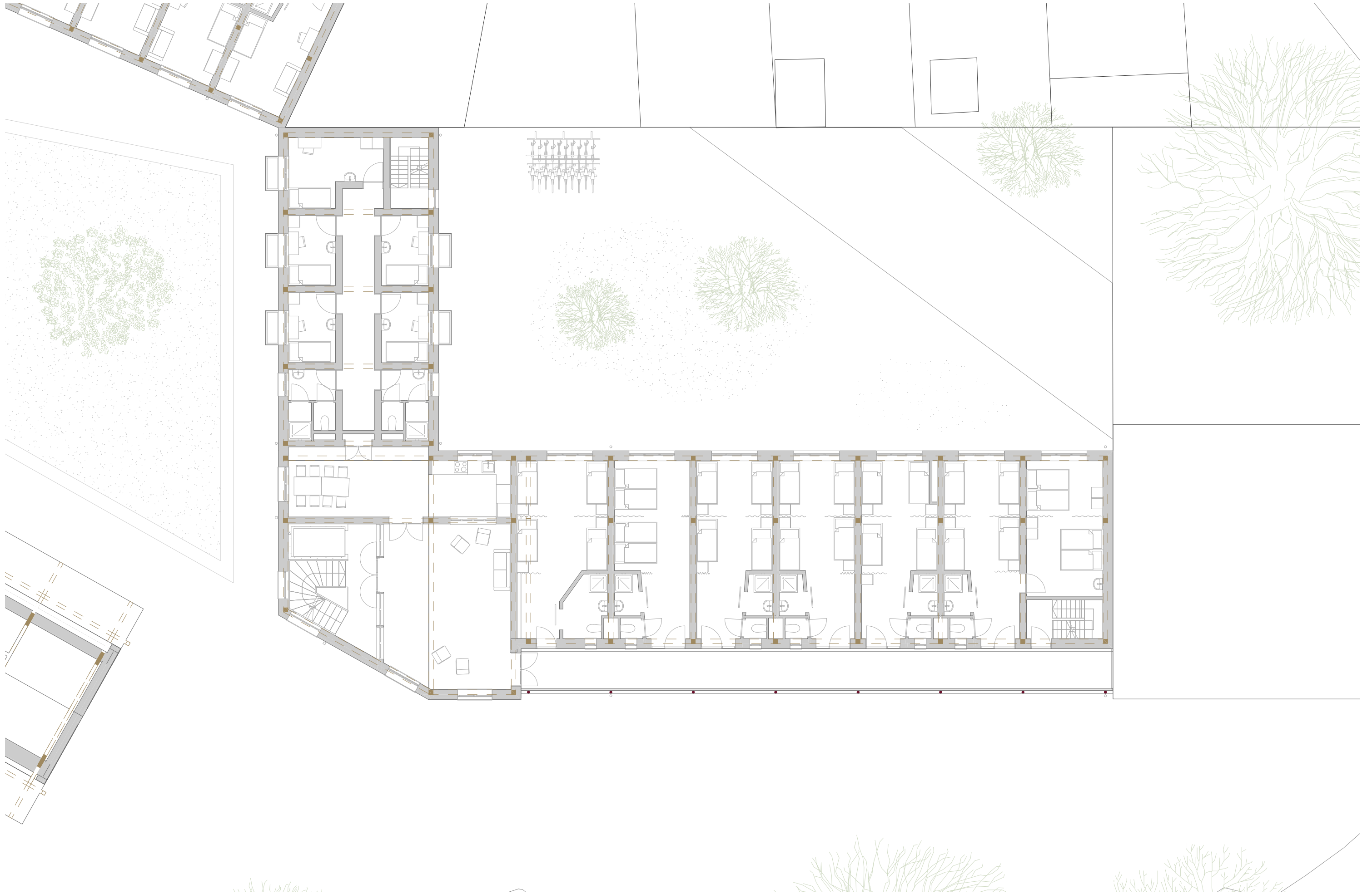
First Floor, Homeless Shelter, 1:120
