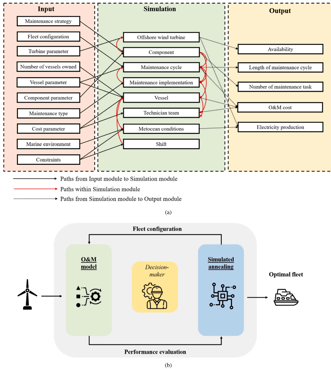
Fig. 2. (a) Schematic diagram of the developed O&M model based on discrete event simulation methods. (b) Flowchart of solving the maintenance fleet mix and size problem.
