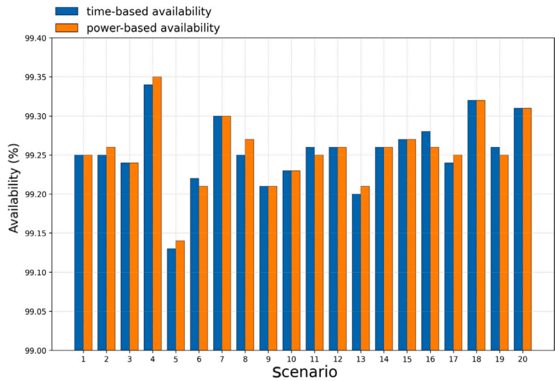
Fig. 8. Time-based and power-based availability of the offshore wind farm.
