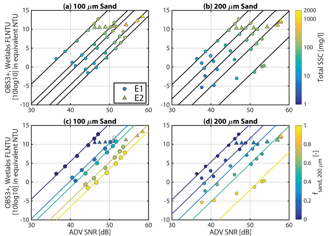
Figure 3. Median acoustic (ADV SNR) and optical backscatter (OBS) as a function of total suspended sediment concentration (a, b) and suspended sand fraction ( f_{\text{sand}} ) in the laboratory experiments (c, d). (a, c) Experiments with 100 \mu\text{m} sand. (b, d) Experiments with 200 \mu\text{m} sand. Data from Experiment 1 (E1) measured with a Wetlabs FLNTU are marked with circles ( n = 30 ), while data from Experiment 2 (E2), measured with an OBS-3+, are marked with triangles ( n = 7 ). Black and colored lines indicate constant f_{\text{sand}} contours. ADV, acoustic Doppler velocimeter; SNR, signal-to-noise ratio.
