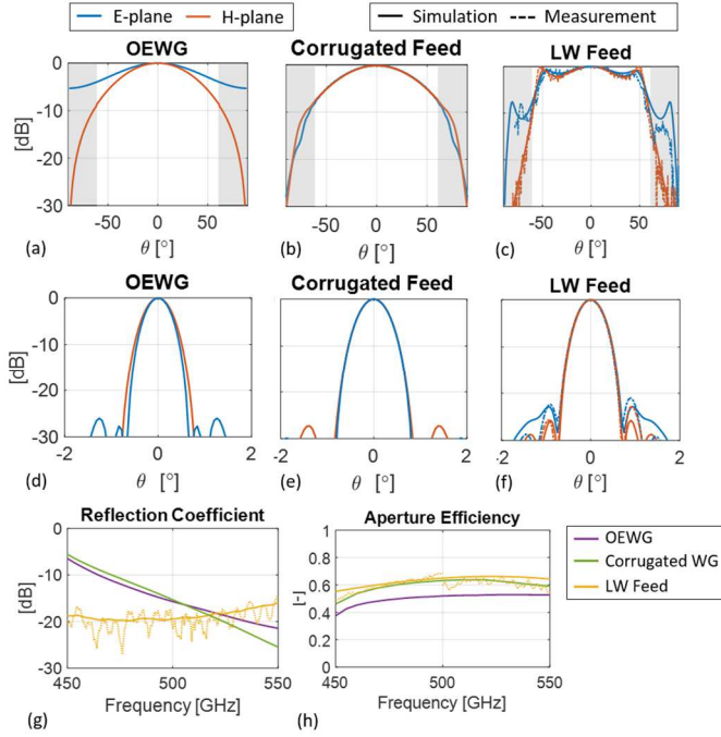
Fig. 2. Feed performance comparison. (a-c) Feed patterns at 500 GHz (E- and H-plane cuts) for, respectively, the OEWG, corrugated WG and LW feed. (d-f) Lens patterns at 500 GHz, (g) reflection coefficient and (h) aperture efficiency of the lens antenna.
