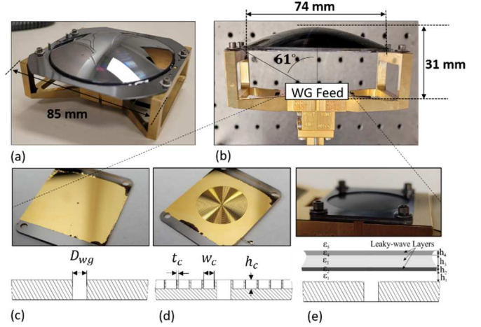
Fig. 1. Low profile lens antenna and WG feeds under investigation. (a) Bird's eye view of the assembled lens antenna. (b) Side-view of the assembled lens antenna; indicated is the position of the WG feed. (c) Benchmark OEWG. (d) Corrugated WG. (e) LW feed.
