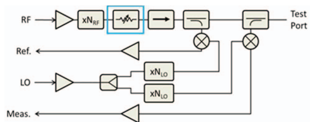
Fig. 1 - Internal scheme block of a frequency extender
