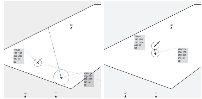
(a) Tangent relative track line (b) CPA of 5 NM
