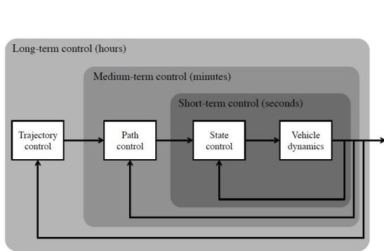
Figure 5.1: Vehicle locomotion control as a multi-loop control problem. [34]
