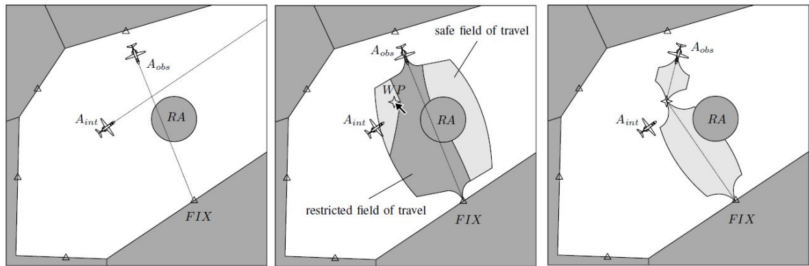
(a) Two conflicting aircraft and a re- (b) The TSR and placement of an inter- (c) Resulting trajectory for the observed restricted airspace mediate waypoint aircraft
