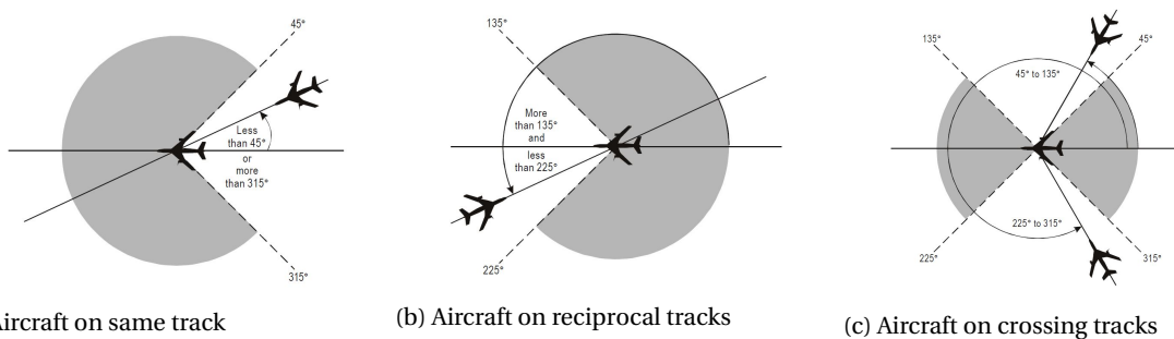
Figure 3.1: Track definitions as defined by ICAO [21]
