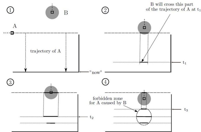
Figure 5.15: Detection of a forbidden zone in the TSD of aircraft A, caused by aircraft B when both trajectories are in the horizontal plane [33]
