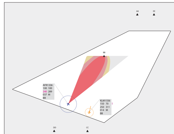
(b) A two-aircraft conflict situation and superimposed 10 kts speed reduction
