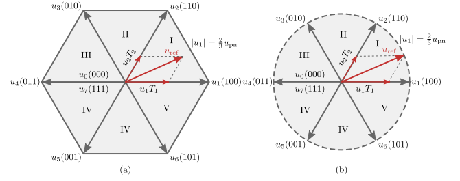
Fig. 3. The space-vector diagram for (a) the traditional PWM methods, (b) the studied two-phase-clamped DPWM.
