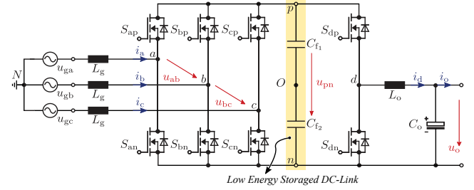
Fig. 1. Circuit topology for three-phase quasi-two-stage buck-type rectifier.
