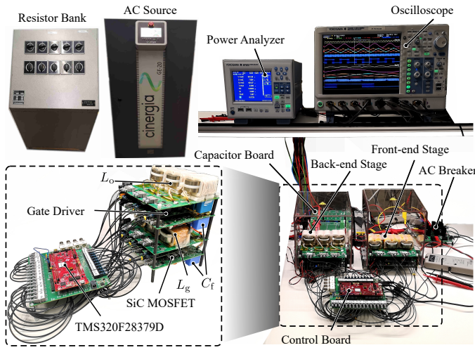
Fig. 17. Experimental setup.
