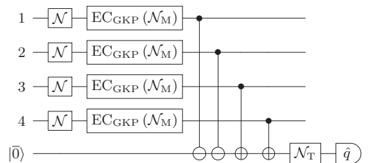
FIG. 7. A single round of error correction for a Z-check for the toric-GKP code in Fig. 6, on oscillators numbered 1 to 4. The GKP error correction unit is given in Fig. 1, |\bar{0}\rangle is a +1 eigenstate of Z and S_p . The inverse CNOT which induces the transformation q_{\text{target}} \rightarrow q_{\text{target}} - q_{\text{control}} (while p_{\text{control}} \rightarrow p_{\text{control}} + p_{\text{target}} ) is denoted using a \ominus at the target qubit instead of a \oplus . A parallel execution of the CNOTs for the X -checks is possible in the toric code.
