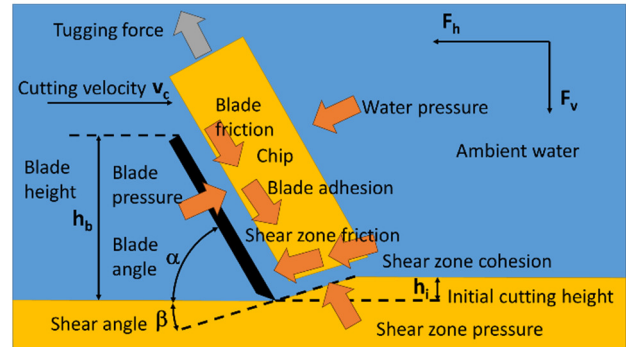
Figure 3 Cutting forces on a clay chip
