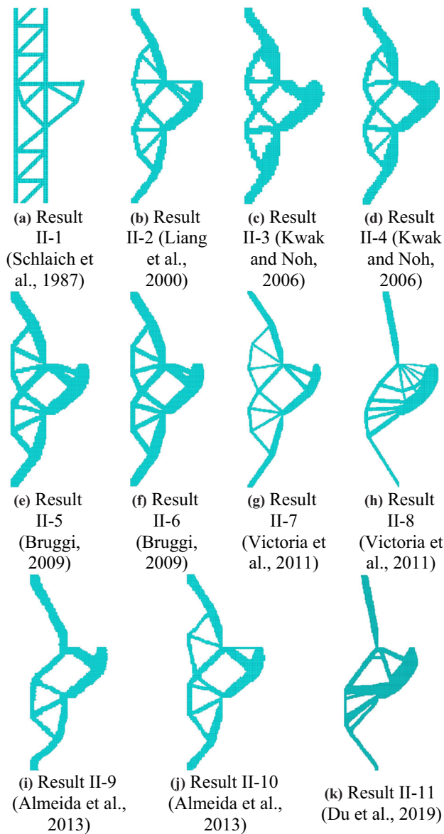
FIGURE 18 Case II: Corbel
