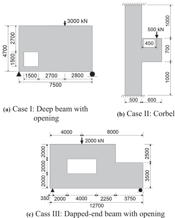
FIGURE 15 Basic information of three cases (mm)
