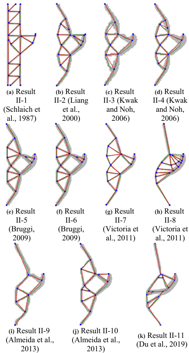
FIGURE A3 Extraction results of Case II: Corbel
