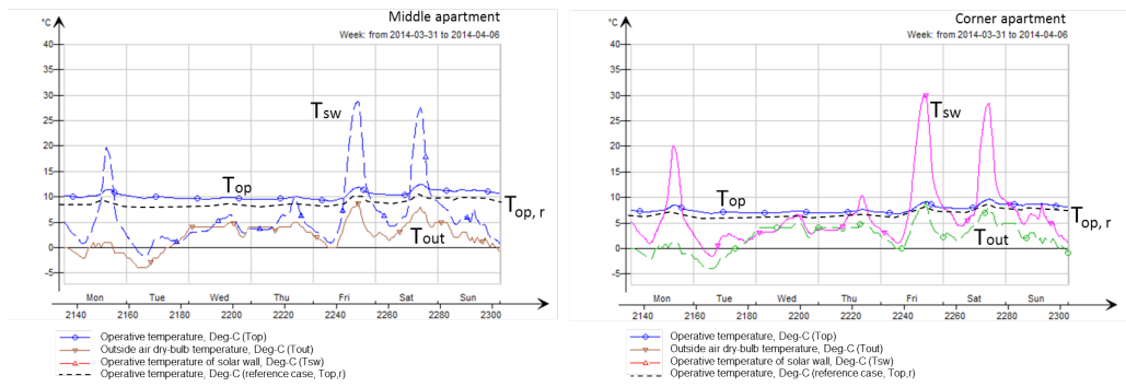
FIG. 8 Temperature profiles, solar wall, week 14 (Mar, 31 to Apr, 06) for the middle apartment (left) and corner apartment (right): Operative temperature T_{op} in adjacent apartment rooms, T_{sw} in solar wall, compared to outdoor temperature T_{out} and old indoor temperature T_{op,r} .
