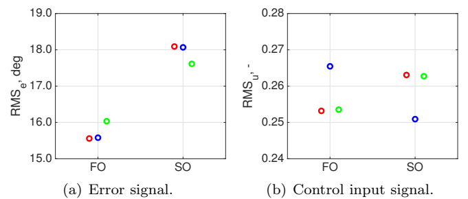
Fig. 4. Root mean square of e and u .
