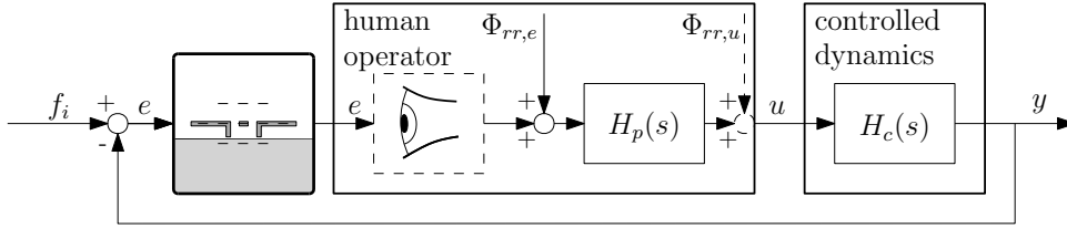
Fig. 1. Control diagram of a manual tracking task.
