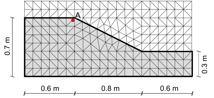
Figure 1: Cross section of 3D slope geometry and mesh (based on Hicks and Wong 1988).
