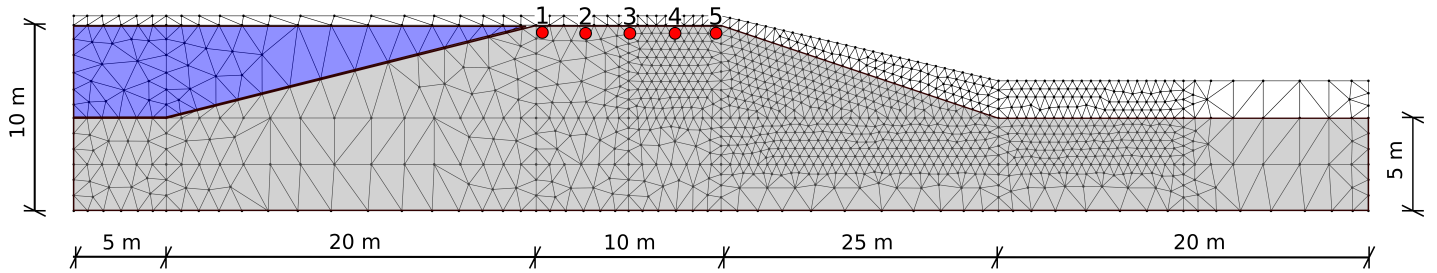
Figure 3: Cross section of dike geometry and mesh.
