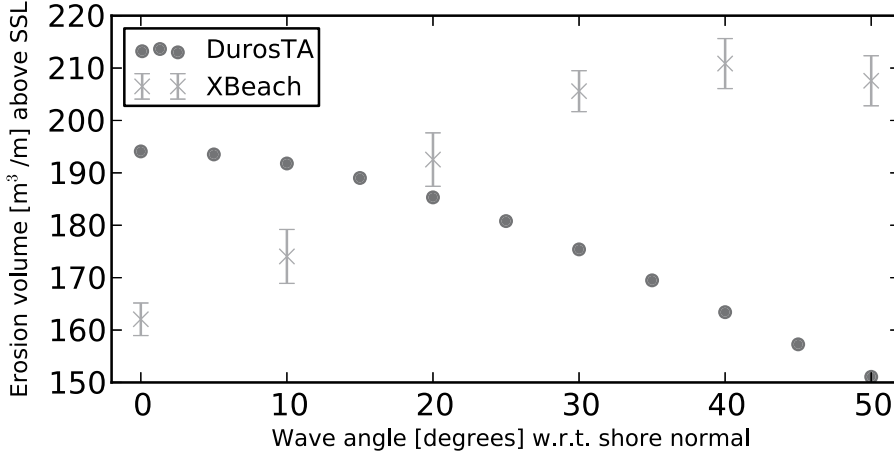
Figure 3.9: DUROSTA and XBEACH erosion volume above storm surge level (SSL) as function of the incident wave angle. The errorbars around the XBEACH results represent the 95 % confidence intervals.
