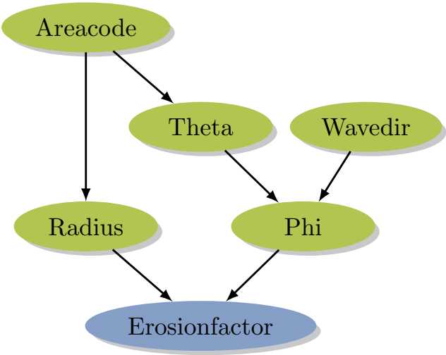
Figure 4.17: Overview of Bayesian Network for wave obliquity and coastline curvature.
