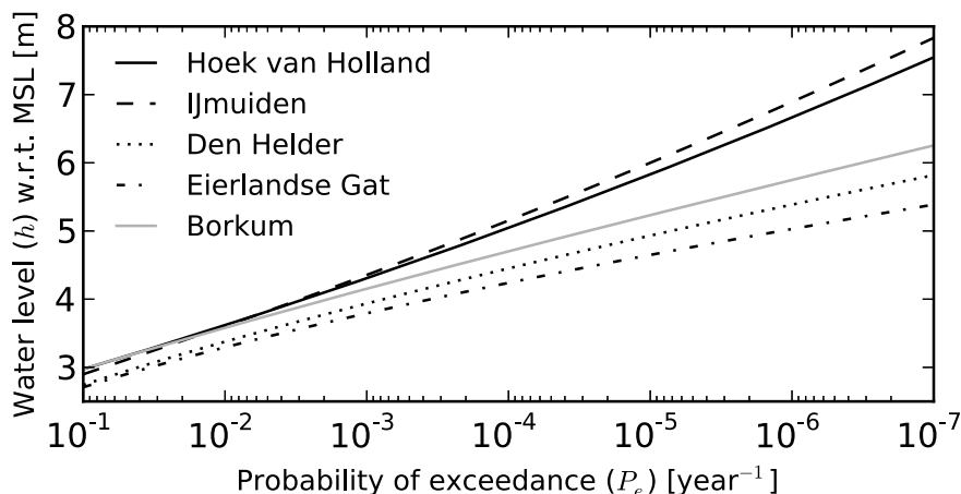
Figure 5.2: Water level as function of probability of exceedance for 5 stations along the Dutch coast.
