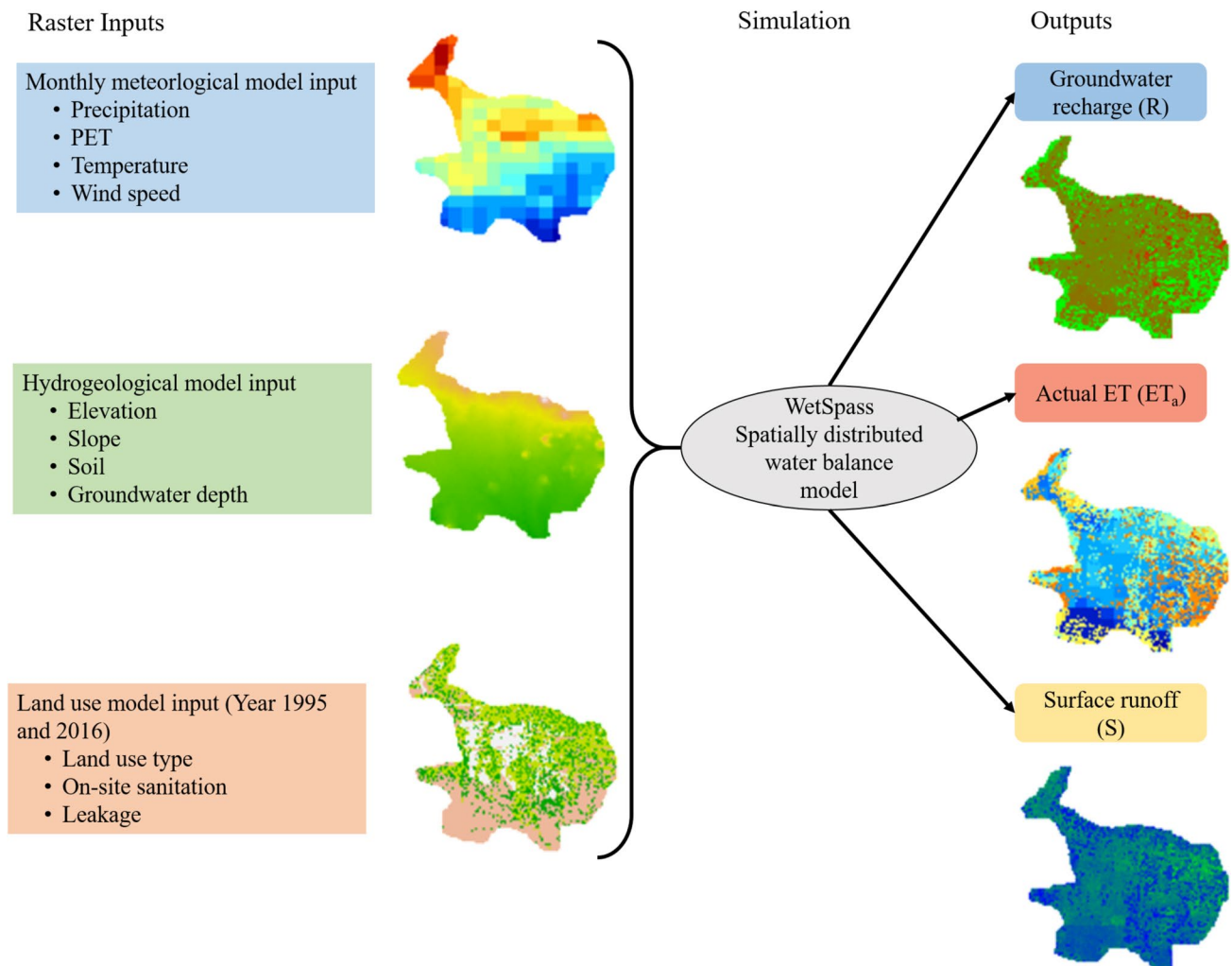
Fig. 2 Conceptual diagram of the WetSpa model, including raster input and output variables
