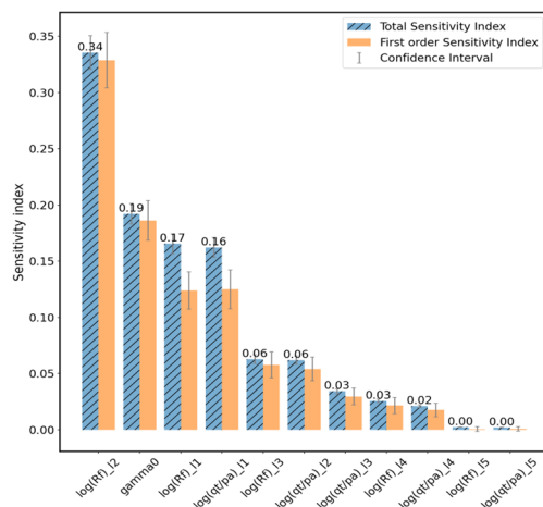
Figure 11. ST and S1 of all parameters (power sample= 12).
