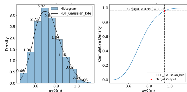
Figure 10. Settlement probability.
