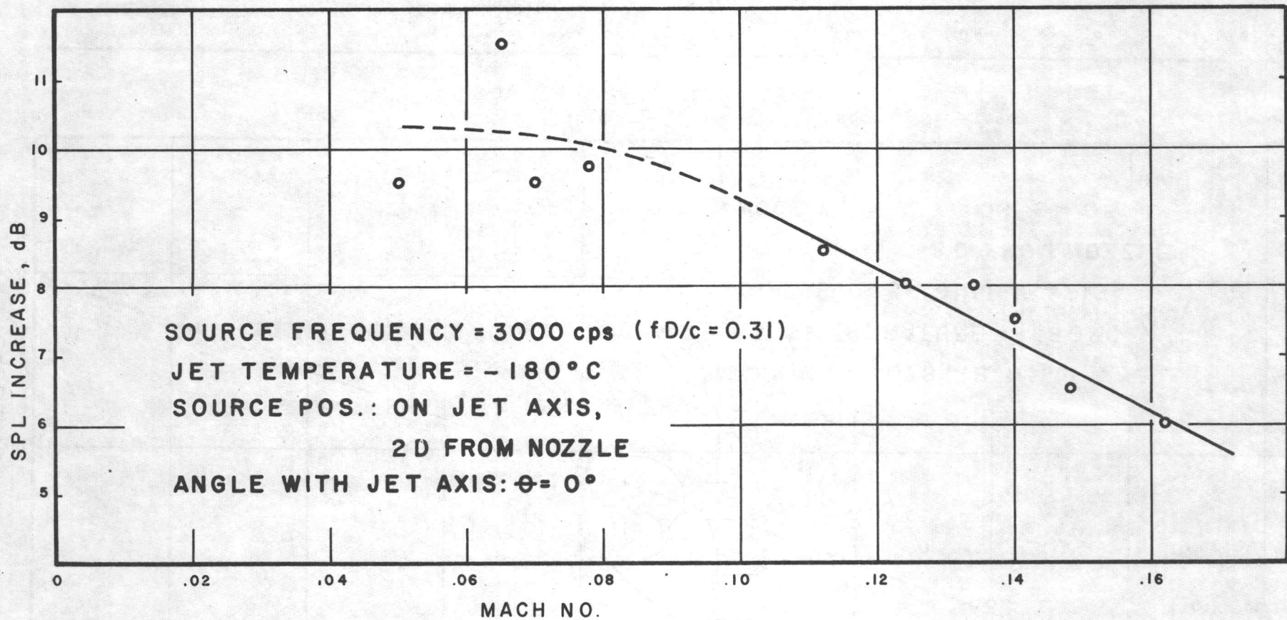
FIG.21. VELOCITY DEPENDENCE OF REFRACTION FOR NITROGEN JET
