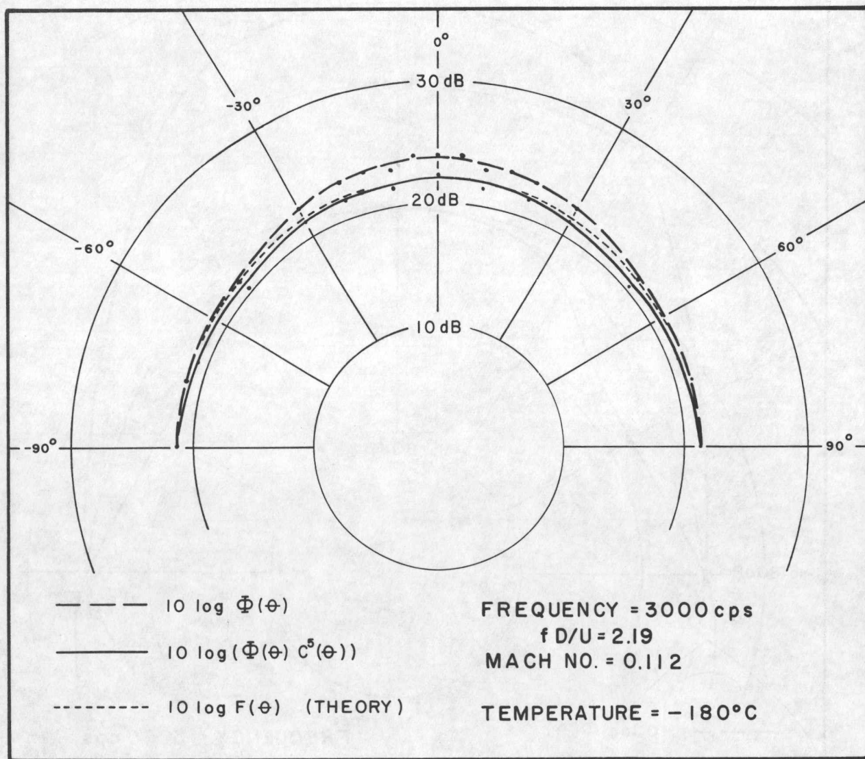
FIG.32. COMPARISON OF EXPERIMENTAL AND THEORETICAL BASIC DIRECTIVITY
