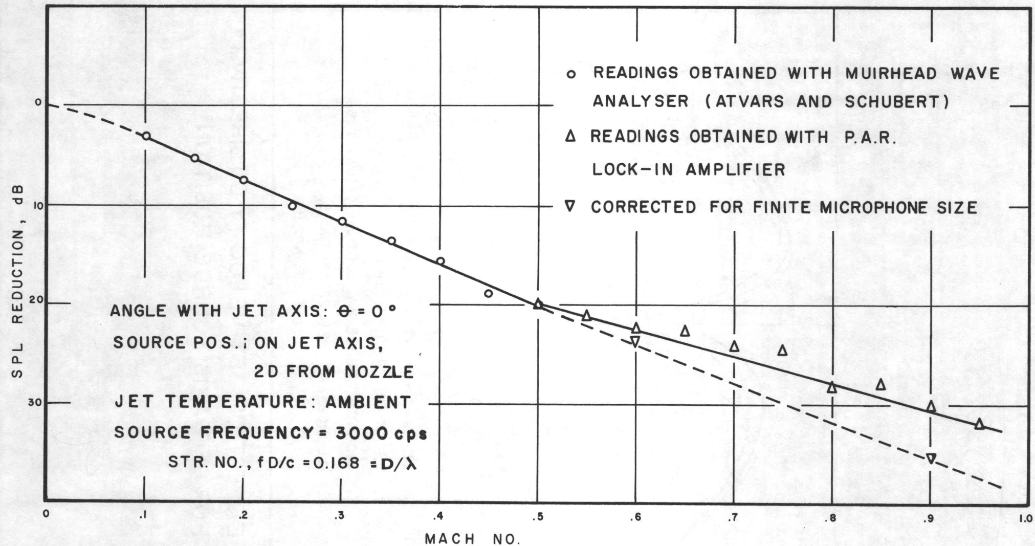
FIG. 7. VELOCITY DEPENDENCE OF REFRACTION
