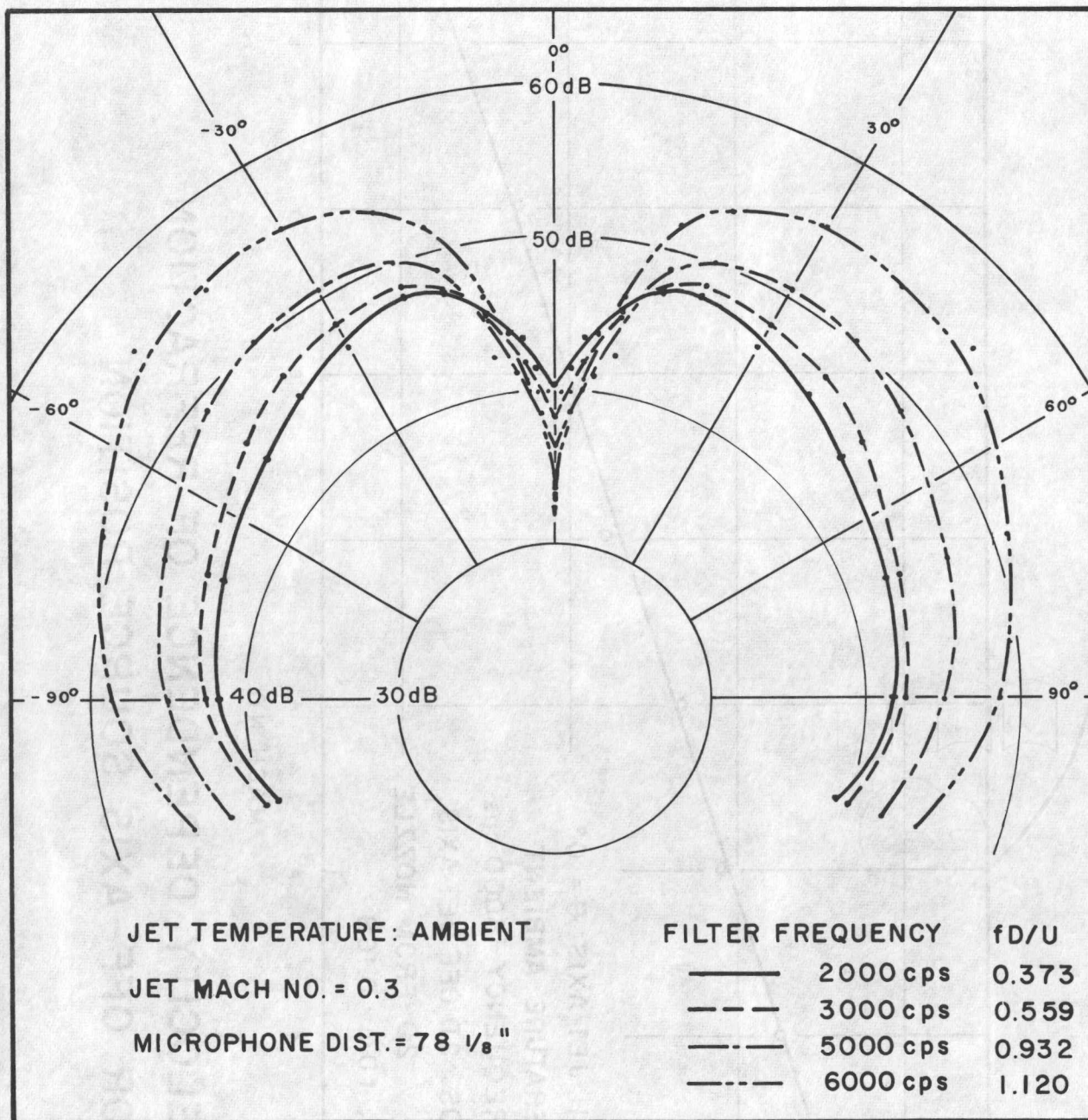
FIG.10. JET NOISE DIRECTIVITY FOR AIR JET
