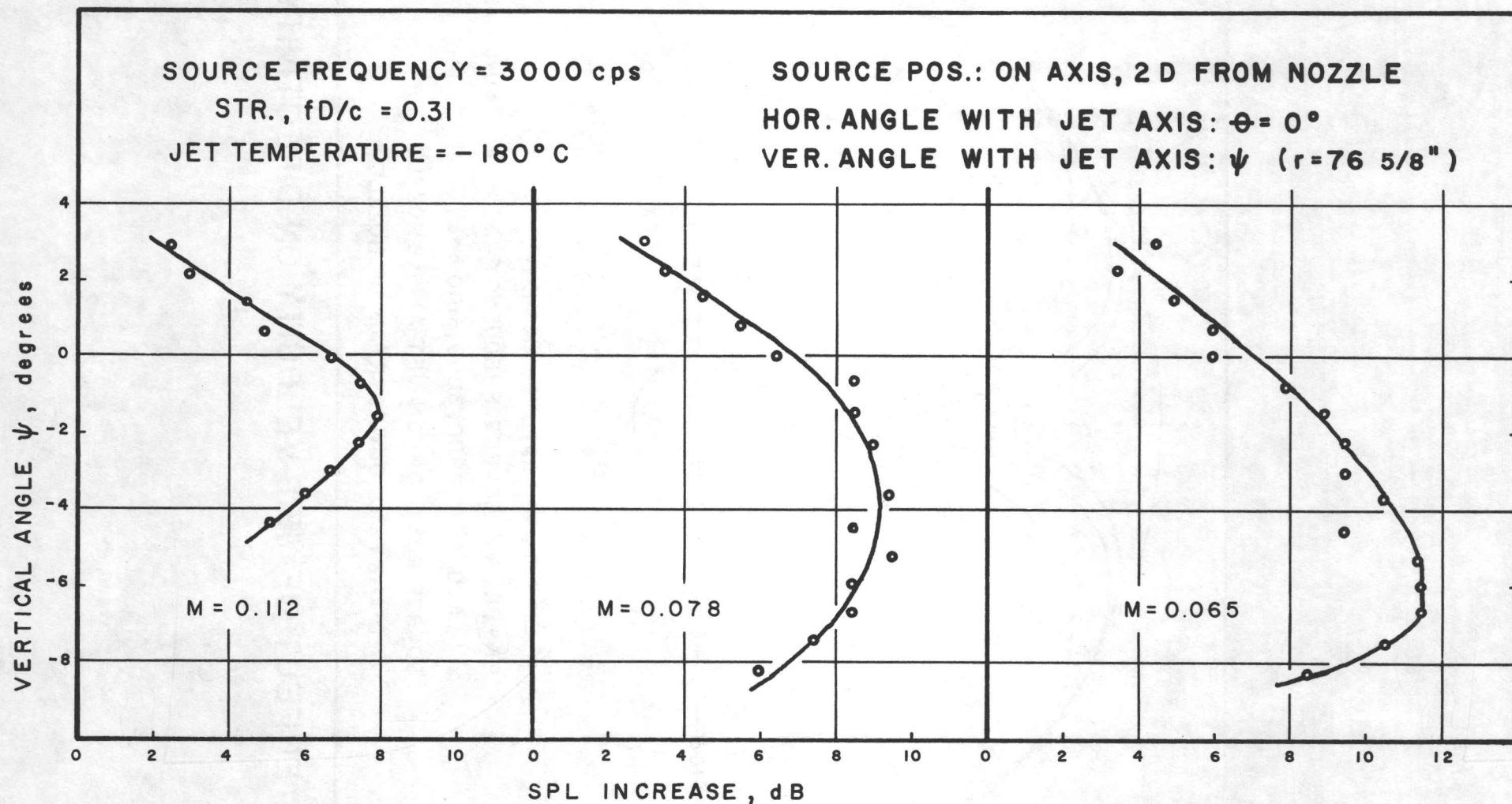
FIG.5. VELOCITY DEPENDENCE OF DROOP OF JET
