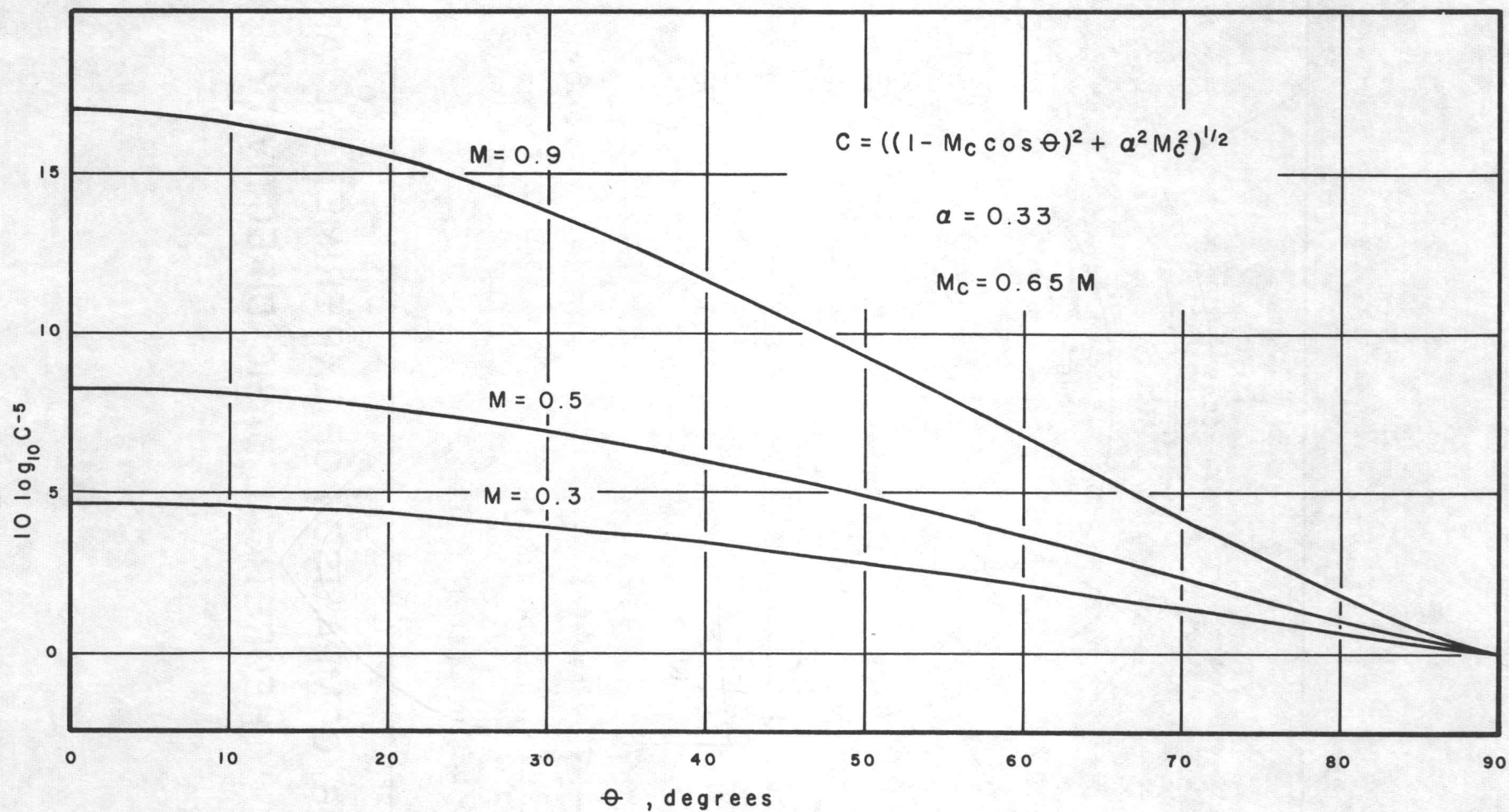
FIG.25. CONVECTION DIRECTIVITY FACTOR
