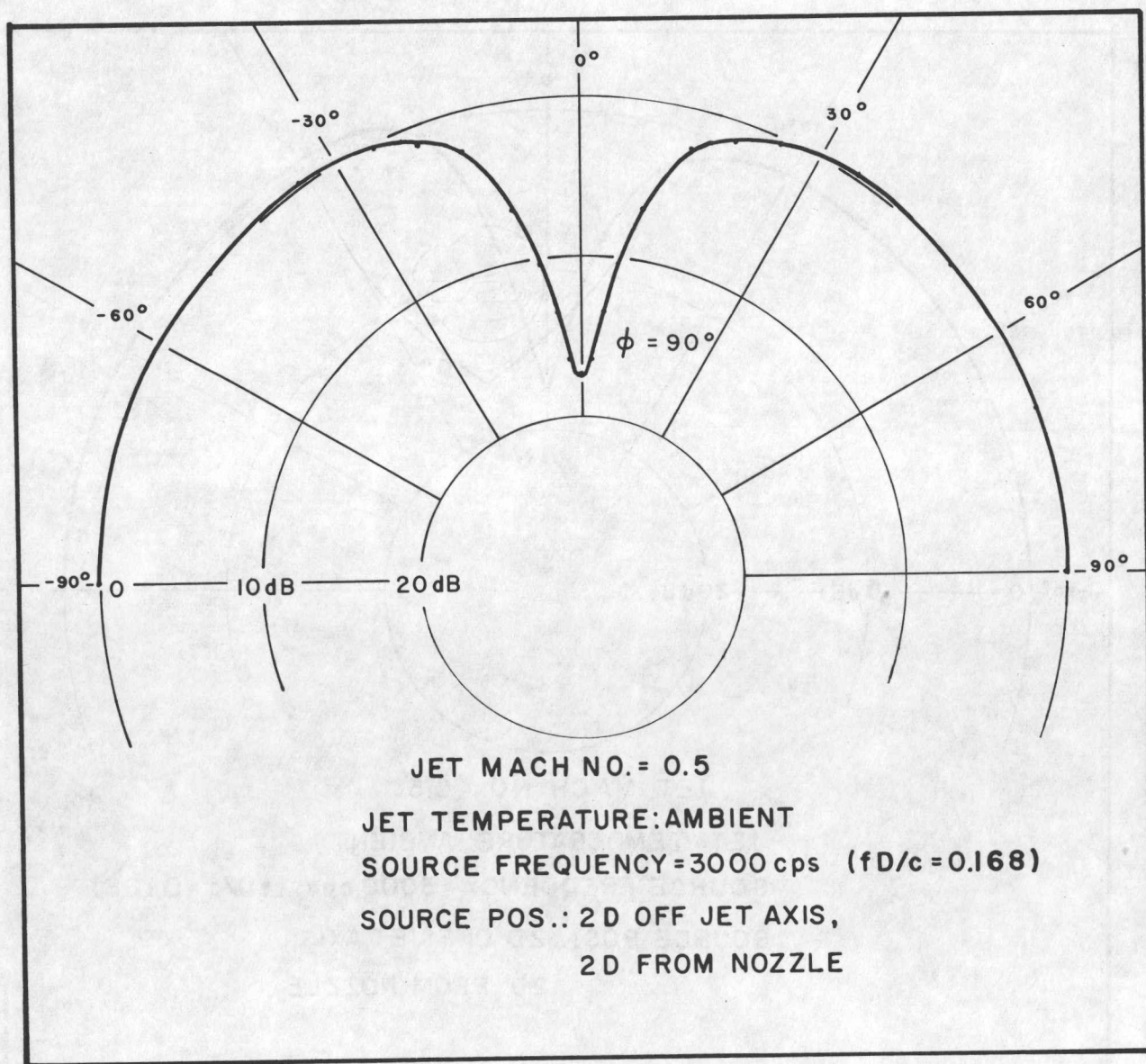
FIG. 18. DIRECTIVITY PATTERN FOR \Phi = 90^\circ
