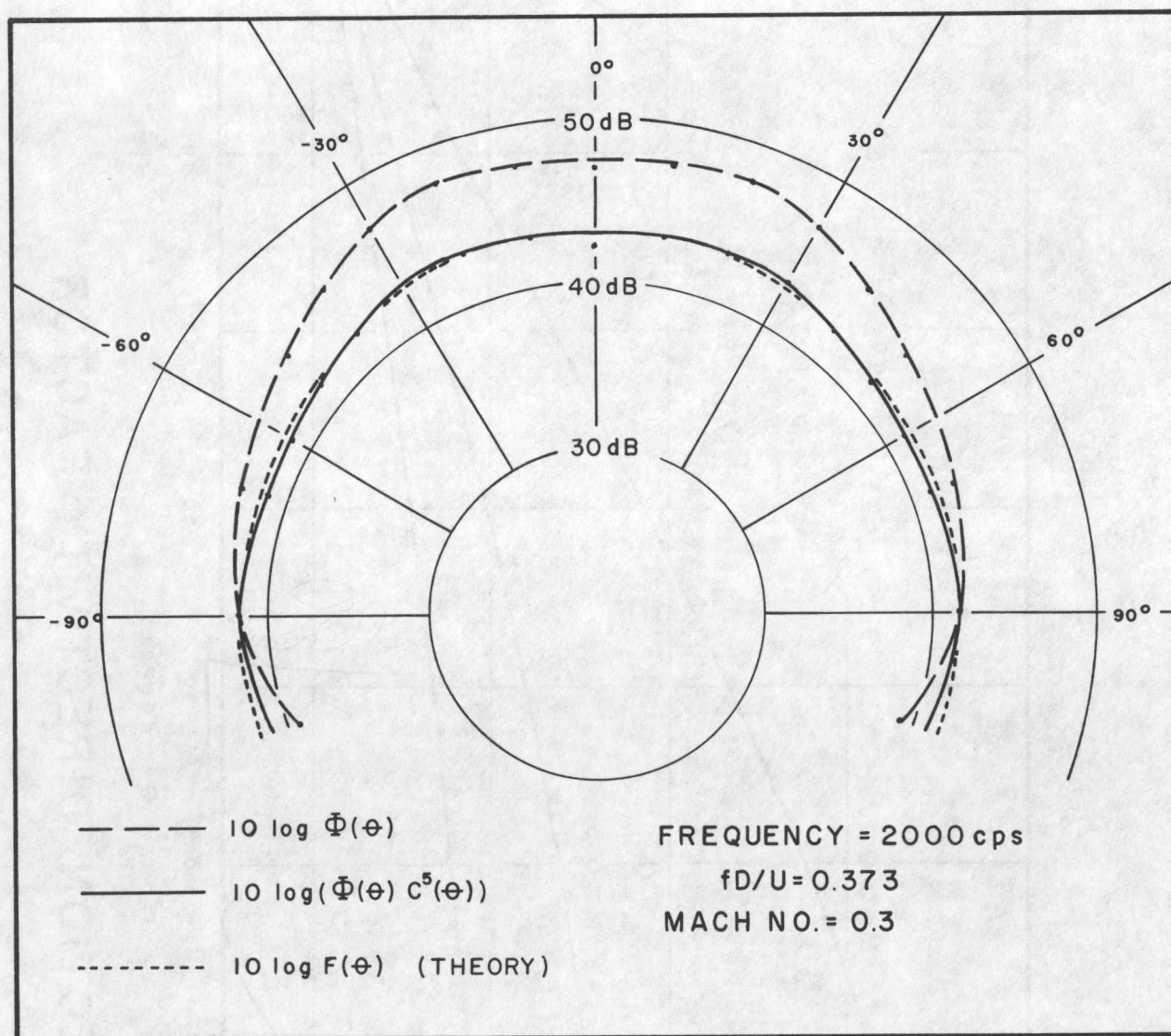
FIG.26. COMPARISON OF EXPERIMENTAL AND THEORETICAL BASIC DIRECTIVITY
