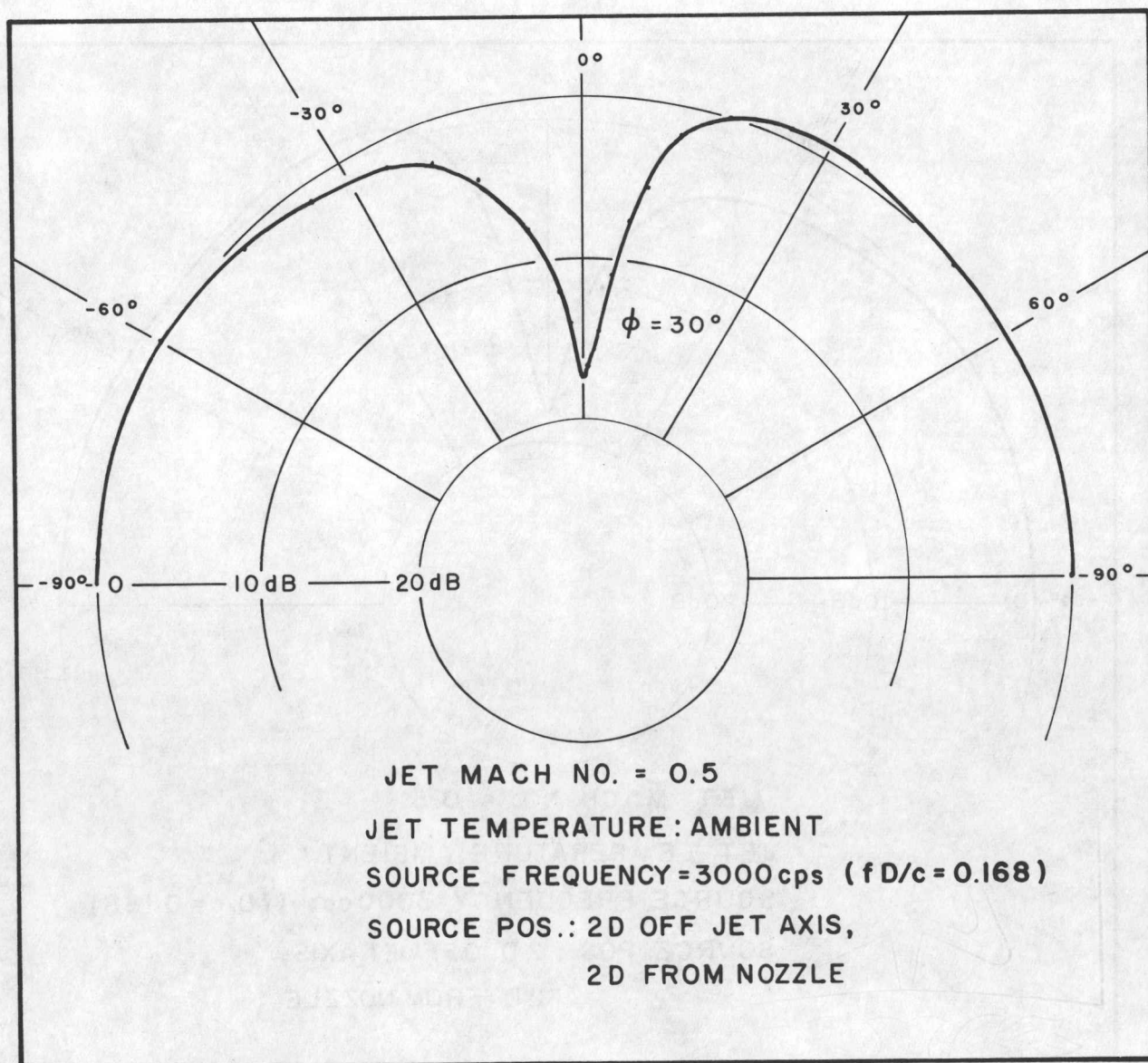
FIG. 16. DIRECTIVITY PATTERN FOR \Phi = 30^\circ
