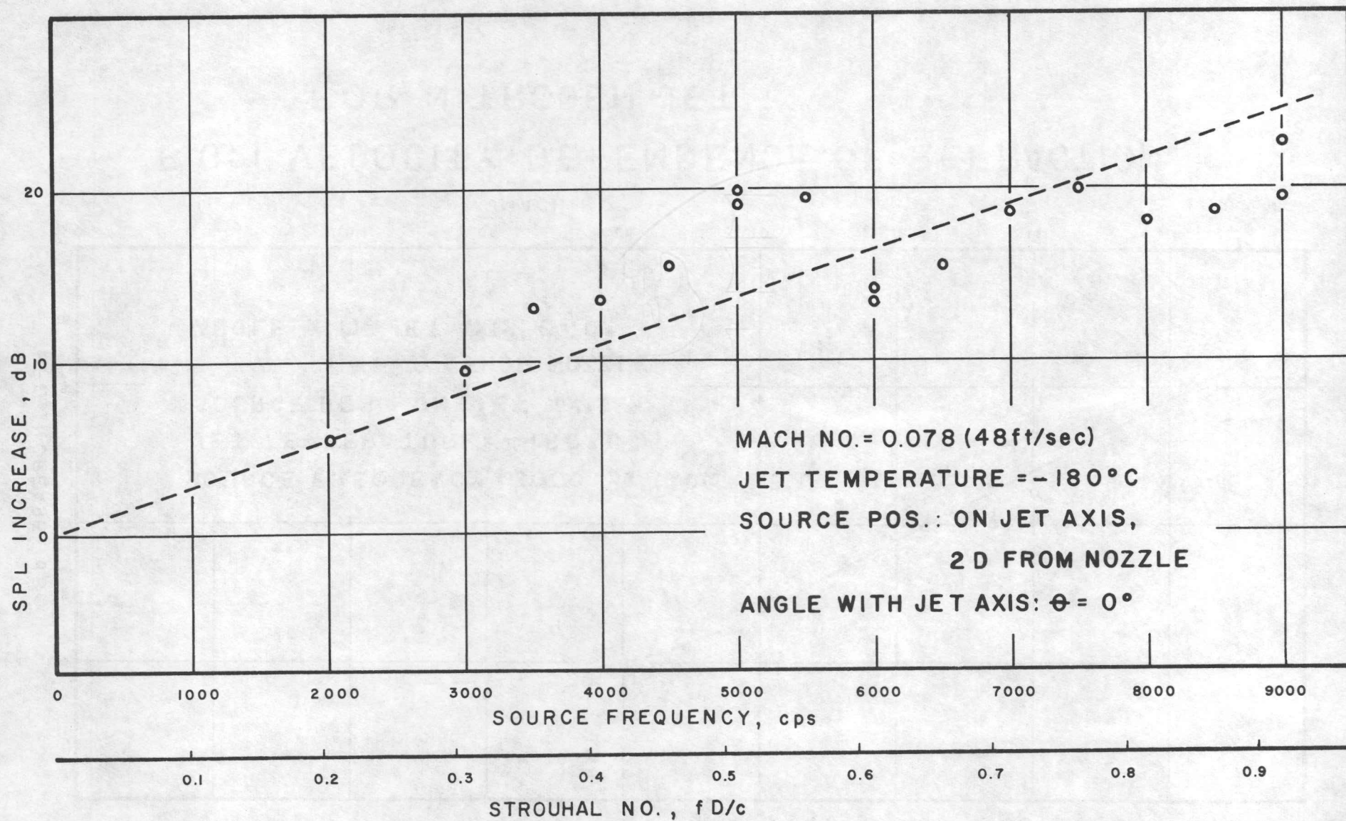
FIG.22. FREQUENCY DEPENDENCE OF REFRACTION FOR NITROGEN JET
