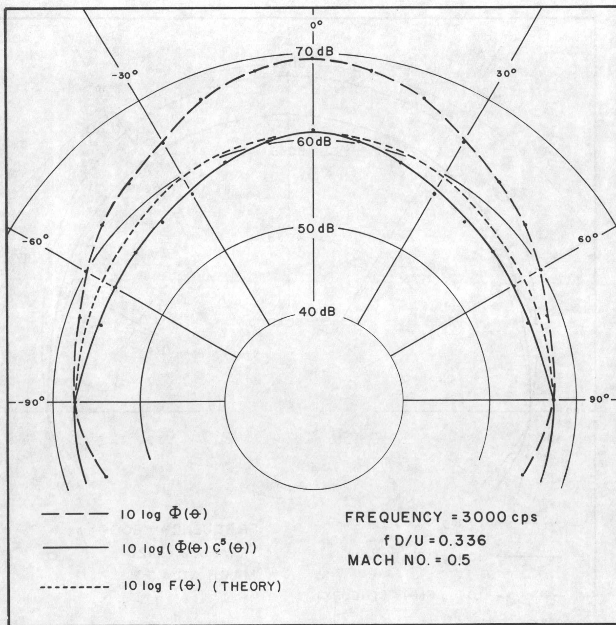
FIG.30. COMPARISON OF EXPERIMENTAL AND THEORETICAL BASIC DIRECTIVITY
