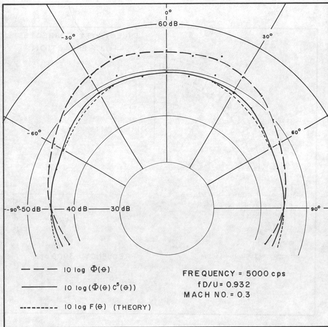
FIG.28. COMPARISON OF EXPERIMENTAL AND THEORETICAL BASIC DIRECTIVITY
