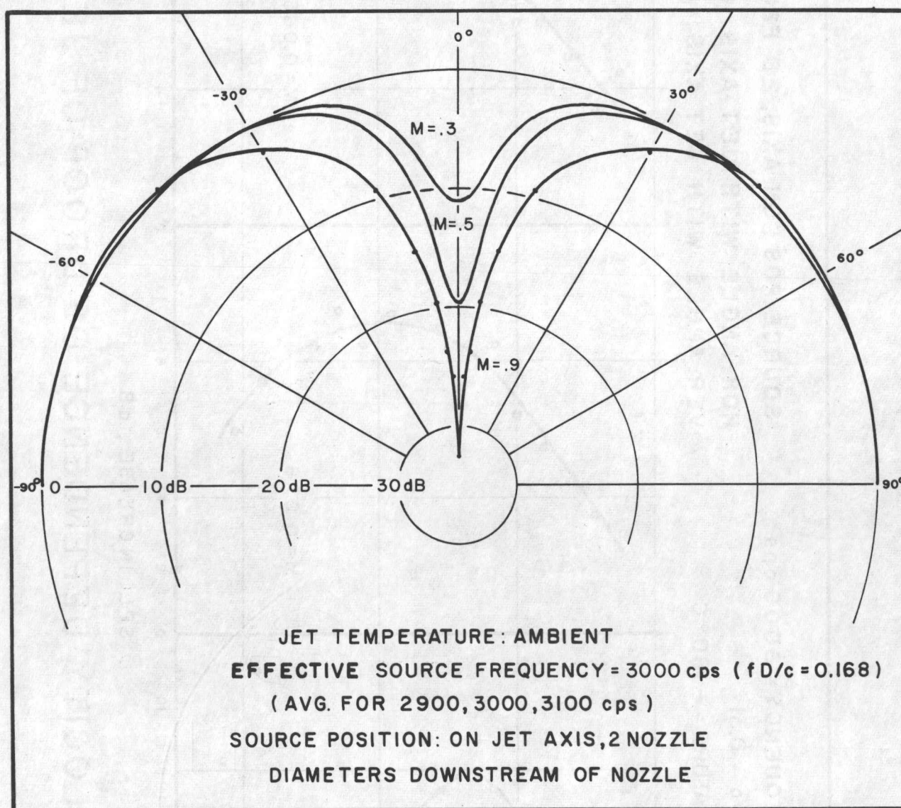
FIG.6. EFFECT OF JET VELOCITY ON DIRECTIVITY
