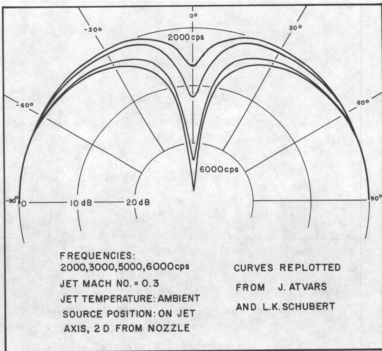
FIG.24.EFFECT OF SOURCE FREQUENCY ON DIRECTIVITY
