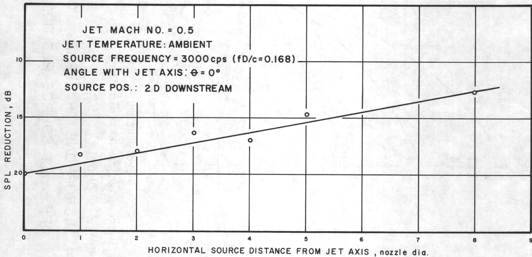
FIG.13. EFFECT OF SOURCE POSITION ON REFRACTION
