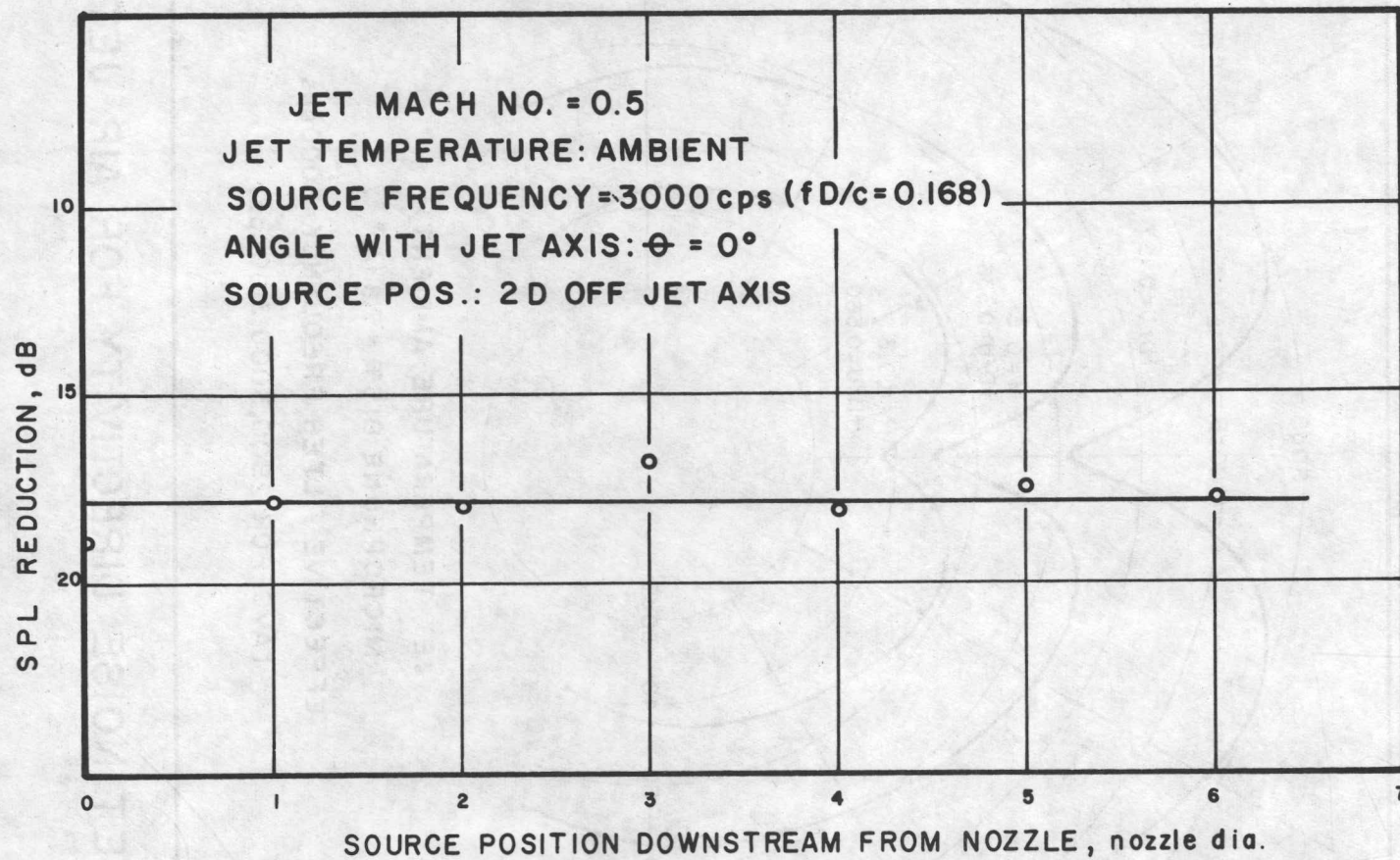
FIG.12. EFFECT OF SOURCE POS. ON REFRACTION
