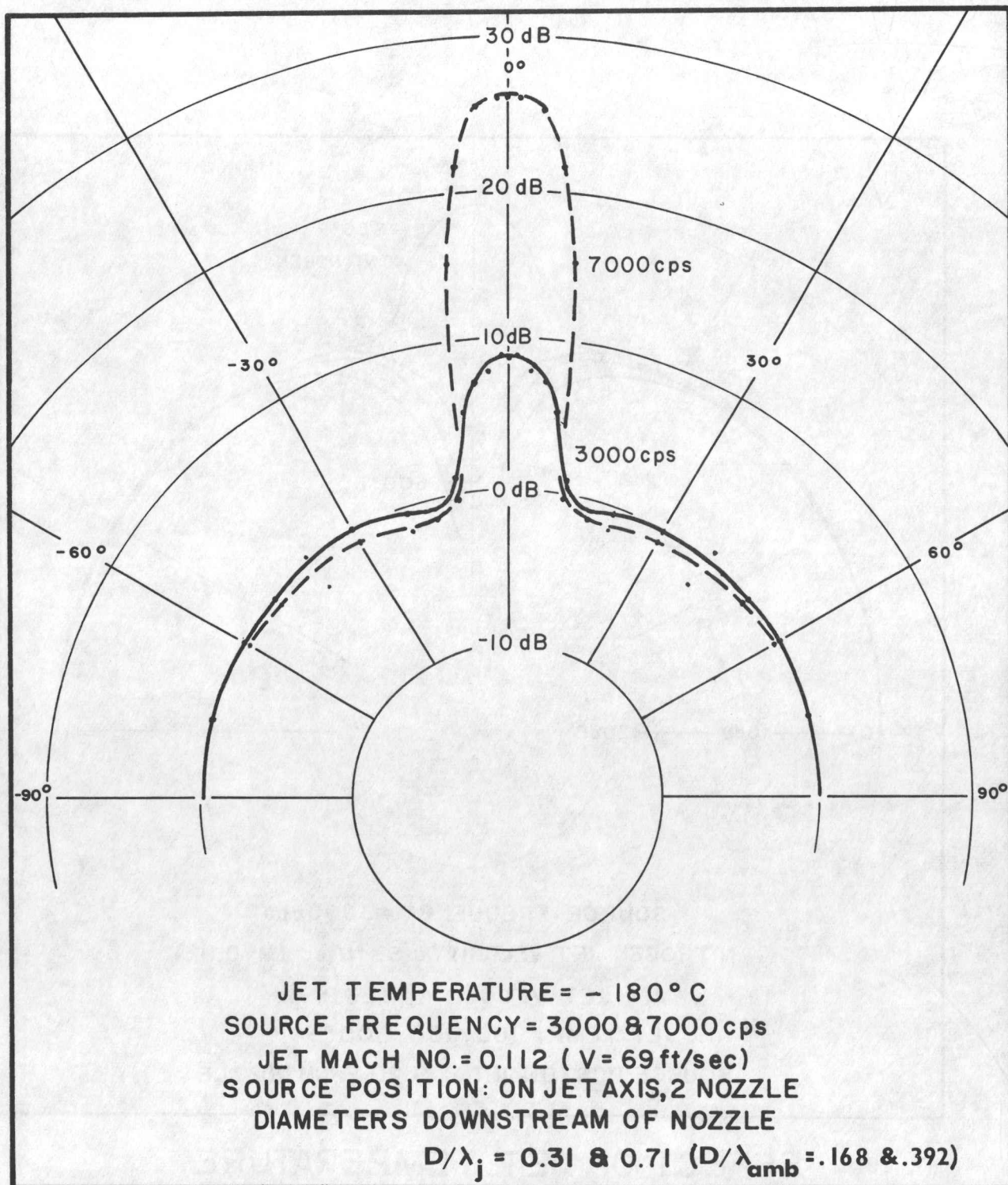
FIG.20.EFFECT OF SOURCE FREQUENCY ON DIRECTIVITY OF NITROGEN JET
