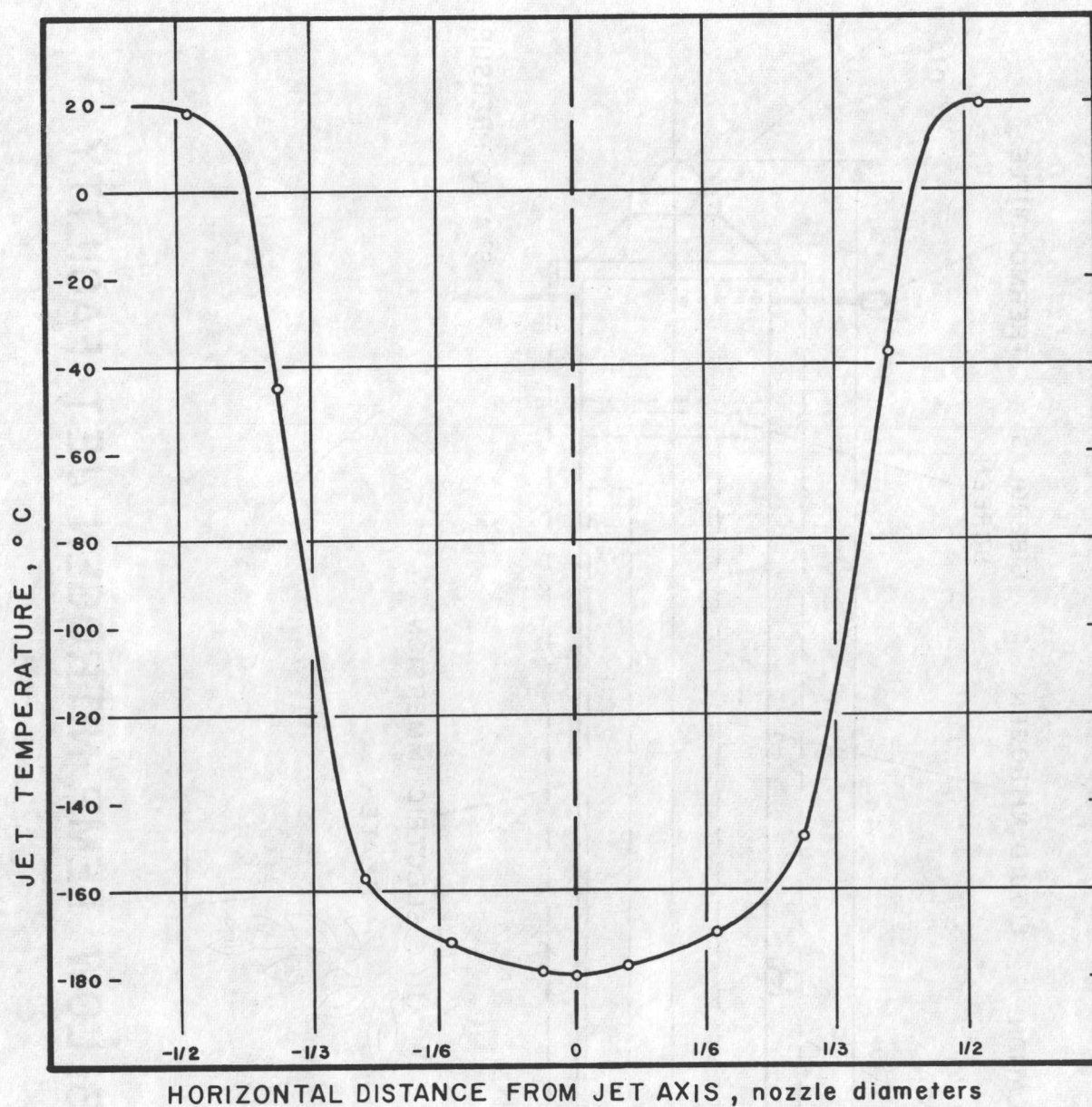
FIG.4. HORIZONTAL TEMPERATURE TRAVERSE \frac{3}{4} " (ID) FROM NOZZLE ; M = 0.078
