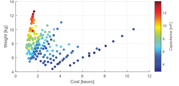
Fig. 5. Weight, costs and capacitance of the feasible DC-link capacitors designs selecting components from [22].
