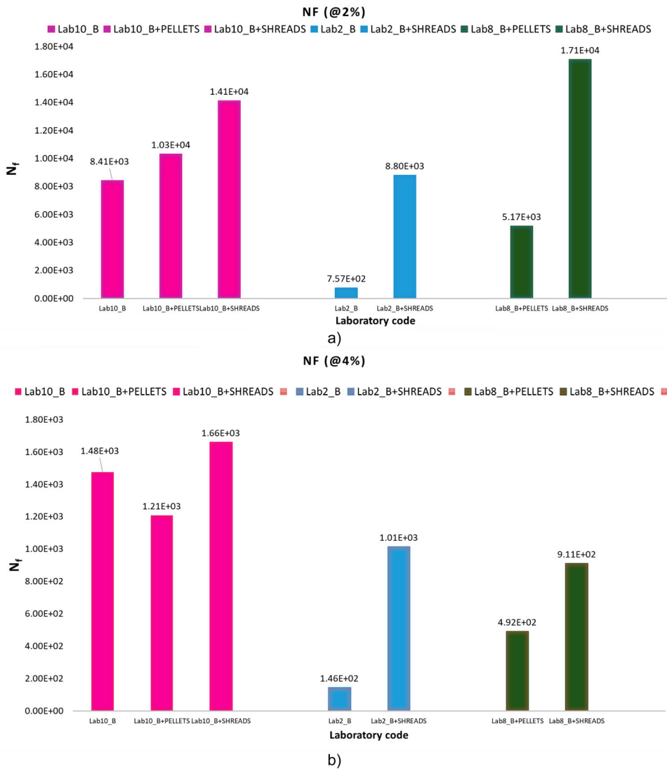
Figure 27. Nf value comparing the three binders: (a) strain level of 2% and (b) strain level of 4%.
