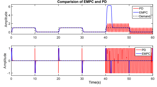
Fig. 21: Comparison of EMPC and PD for G(s) = \frac{1000}{s(s^2 + 60s + 500)(s^2 + 60s + 500)}
