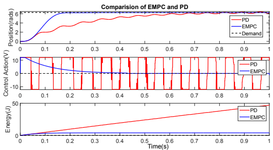
Fig. 42: Comparison of EMPC and PD for under-damped position control of a practical motor system
