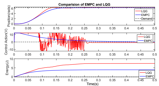
Fig. 44: Comparison of EMPC and LQG for under-damped position control of a practical motor system
