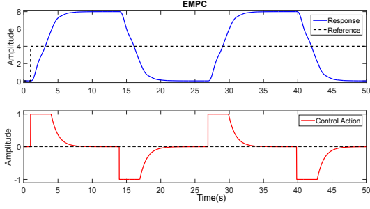
Fig. 15: Simulated Response of H(s) for K'_{sa} = 2K
