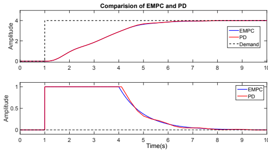
Fig. 24: Comparison of EMPC and PD for under-damped system H(s) = \frac{17}{s(s^2 + 2s + 17)}
