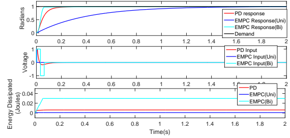
Fig. 29: Comparison of EMPC and PD for well-damped position control of motor for large inertia system J'_l = J_l * 10
