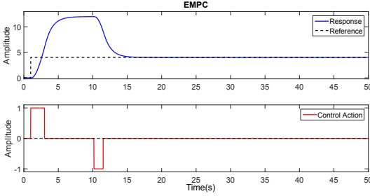
Fig. 9: Simulated Response of G(s) for K'_{sa} > 2K
