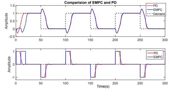
Fig. 22: Comparison of EMPC and PD for G'(s) = \frac{0.5(0.2 - s)}{s(s^2 + 2s + 1)}
