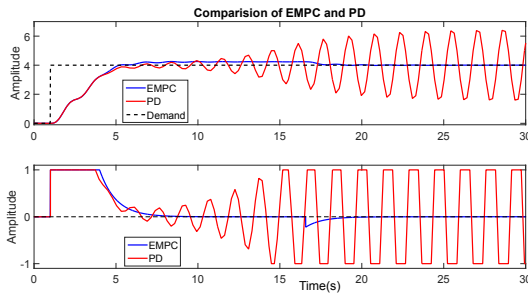
Fig. 25: Comparison of EMPC and PD for under-damped system H'(s) = \frac{17}{s(s^2 + 0.5s + 16.0625)}
