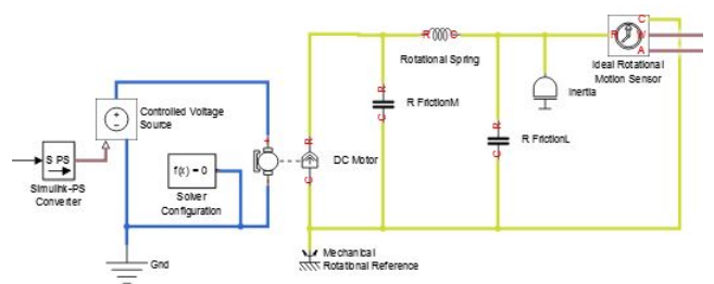
Fig. 38: Simulation model of a load coupled to a motor through a flexible shaft
