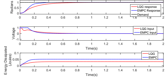
Fig. 37: Comparison of EMPC and LQG for under-damped position control of motor for large inertia system J'_l = J_l * 10
