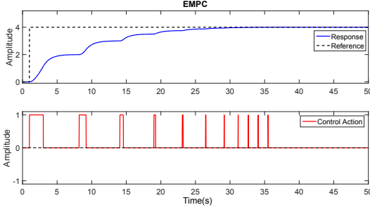
Fig. 2: Simulated Response of G(s) for K'_{sa} < K
