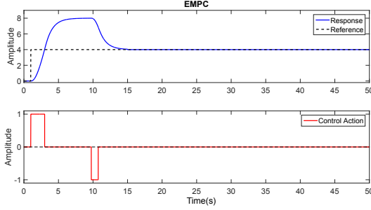
Fig. 8: Simulated Response of G(s) for K'_{sa} = 2K
