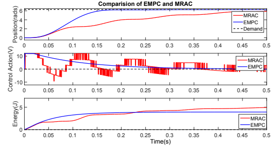
Fig. 43: Comparison of EMPC and MRAC for under-damped position control of a practical motor system
