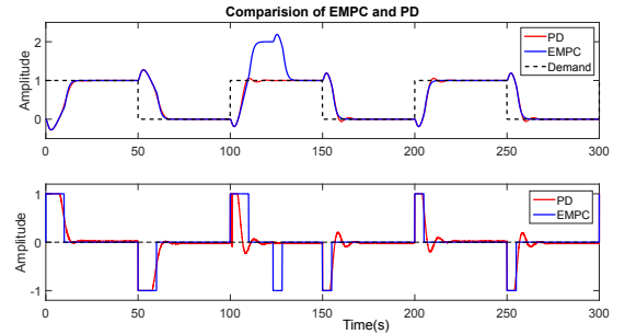
Fig. 23: Comparison of EMPC and PD for G'_1(s) = \frac{0.5(0.4 - s)}{s(s^2 + 2s + 1)}
