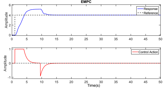
Fig. 18: Simulated Response with OJR for H(s) for K < K'_{sa} < 2K
