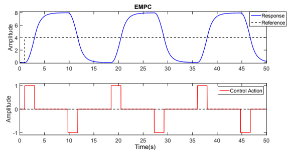
Fig. 4: Simulated Response of G(s) for K'_{sa} = 2K
