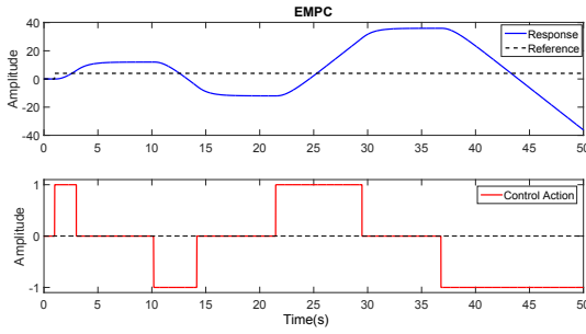
Fig. 5: Simulated Response of G(s) for K'_{sa} > 2K
