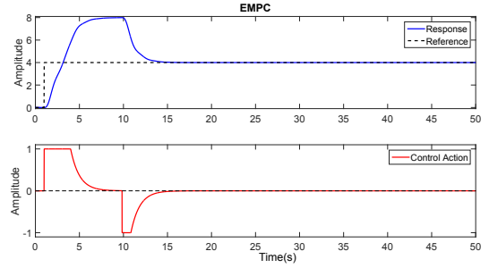
Fig. 19: Simulated Response with OJR for H(s) for K'_{sa} = 2K
