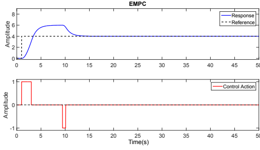
Fig. 7: Simulated Response of G(s) for K < K'_{sa} < 2K
