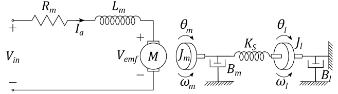
Fig. 26: Model of a DC Motor Position System coupled to a Load with a Flexible Shaft
