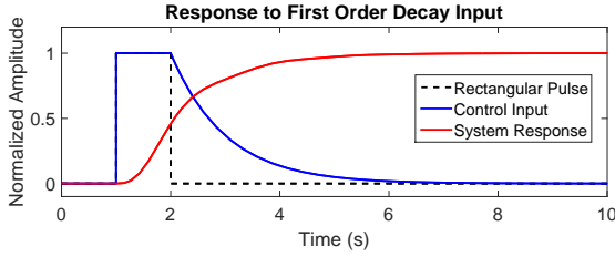
Fig. 11: Response of System H(s) = \frac{17}{s(s^2 + 2s + 17)} to First Order Decay Input [ \alpha = 1 ]
