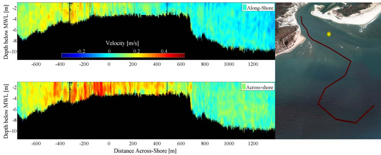
Figure 4. A sampling of the ADCP measured current profiles as SPECT crossed the NRI shoals. This data were taken from Run 13. Shown is the two-dimensional (top) alongshore and (bottom) across-shore flow velocity, where the color scale applies to both figures. On the right, the corresponding SPECT GPS track, with the (0,0) marked in yellow.
