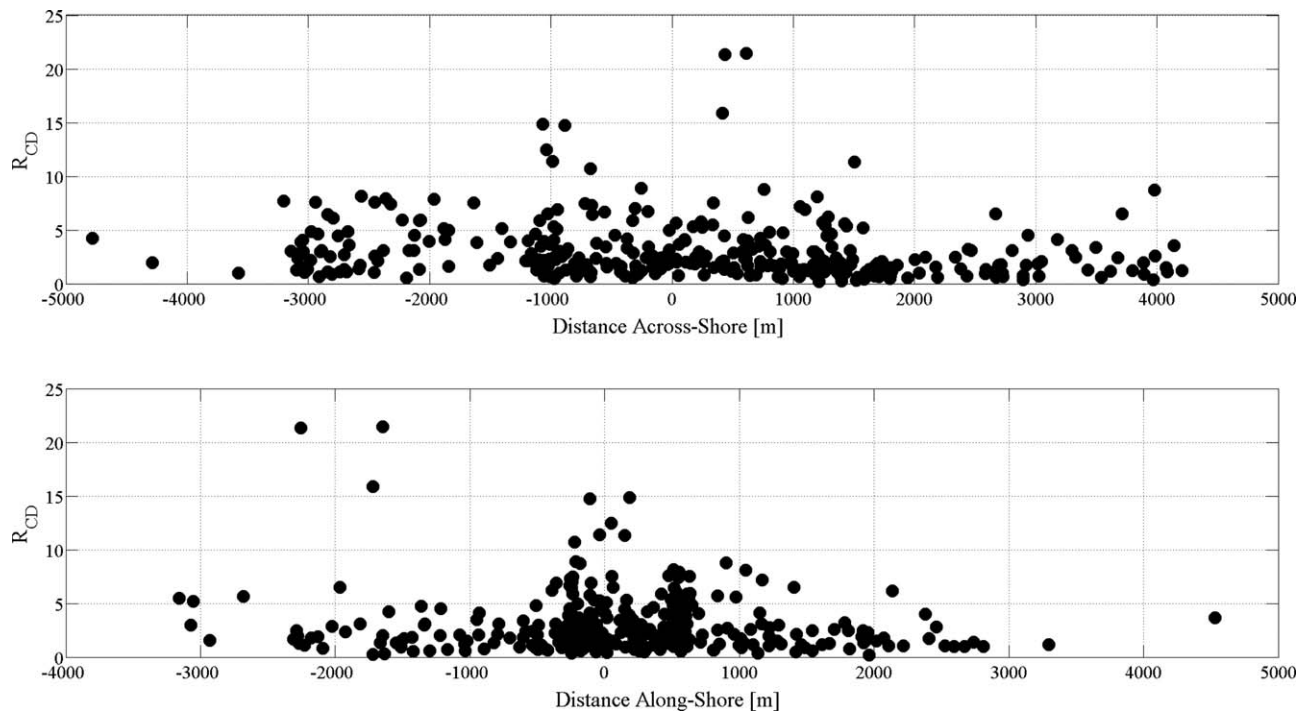
Figure 9. The (top) cross-shore and (bottom) along-shore distribution of the R_{CD} values (equation (12)). Here R_{CD} is defined as the ratio of the drag coefficient calculated from an eddy covariance method to a Smith [1988] algorithm, for any give 5 min segment of data.
