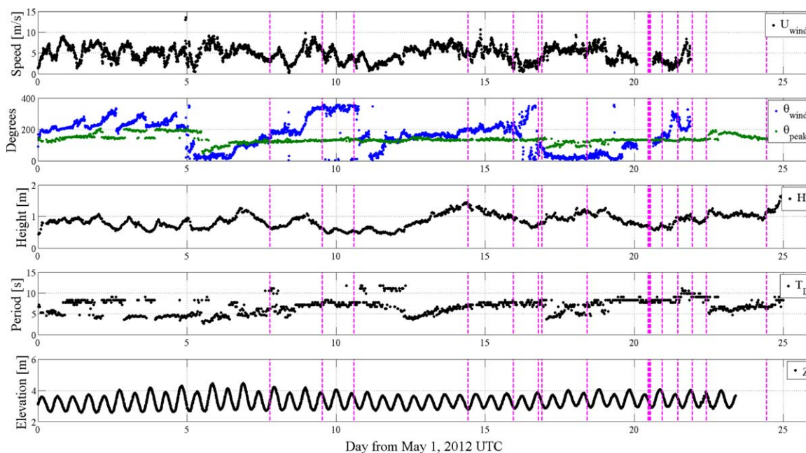
Figure 2. Time series of bulk meteorological and wave data. From top to bottom, U_{wind} is 10 min mean wind speed from an 8 m, land-based tower (location given in Figure 1c as “W”); \theta_{wind} and \theta_{peak} are the wind direction from the wind tower and the peak incident wave direction from an NDBC waverider buoy moored 6 km offshore of NRI, respectively; H_s is the significant wave height from the waverider; T_D is the peak period; and finally, Z is the 5 min mean water surface elevation from a bottom-mounted pressure sensor (location given in Figure 1c as “P”). All wave parameters are calculated over 30 min. Magenta lines mark start times of SPEC runs (Table 1).
