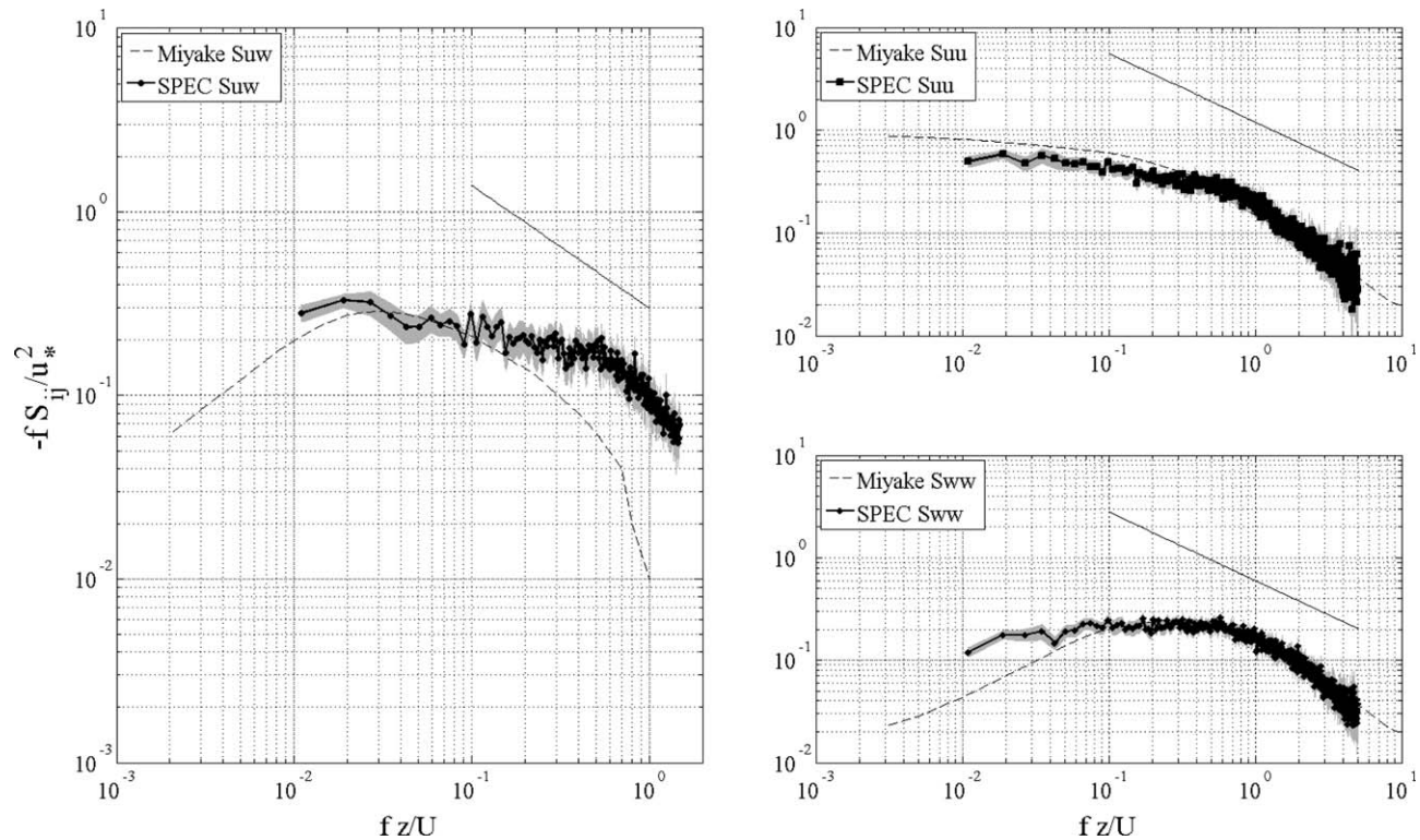
Figure 5. Turbulence spectra results compiled from all SPECT runs. The universal curves of Miyake et al. [1970] and the proposed Kolmogorov -5/3 slope of the inertial subrange (the thin black line) are also given. The shaded area represents the span of the 95% confidence interval calculated over a 30 element bin average. (left) The normalized cospectrum. (right) The normalized spectra for each respective component. The spectral amplitudes were normalized by the shear velocity squared, while z and U are taken as the height above the m.w.l and the corresponding mean wind speed, respectively.
