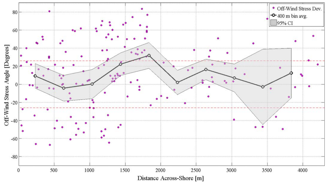
Figure 7. The spatial distribution of observed wind stress angles. The points represent the angle between 5 min means of the along and across-wind components of the wind stress. The solid line, with the open circles, gives the data filtered by a 400 m wide bin average. The shaded region spans the 95% confidence calculated from each bin. The red lines mark the \pm 26^\circ line, which is the cutoff used in Smith [1980] to consider the wind stress in-line with the wind vector.
